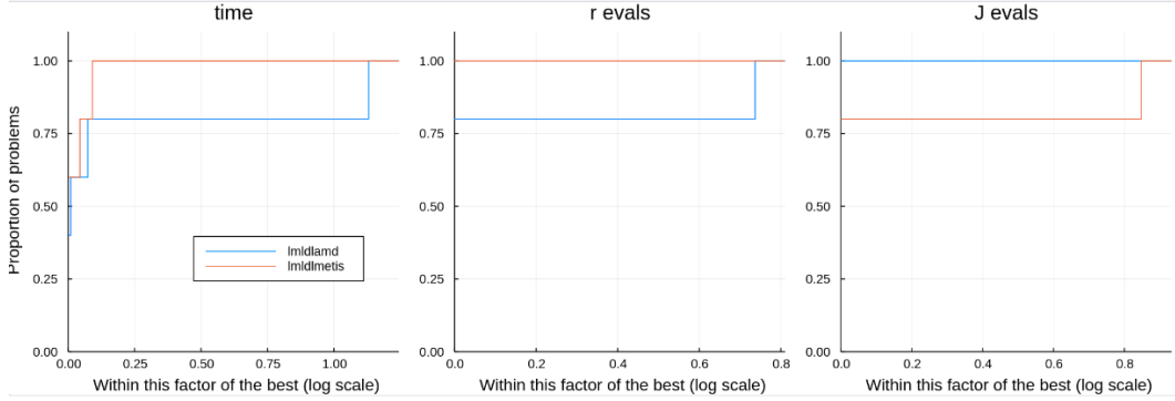
Figure 7: Profile of the LDL version on “big problems”
