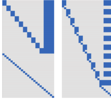
Figure 1: \begin{bmatrix} R \\ \sqrt{\lambda} \end{bmatrix} on the left and P \begin{bmatrix} R \\ \sqrt{\lambda} \end{bmatrix} on the right (Image taken from [20])
