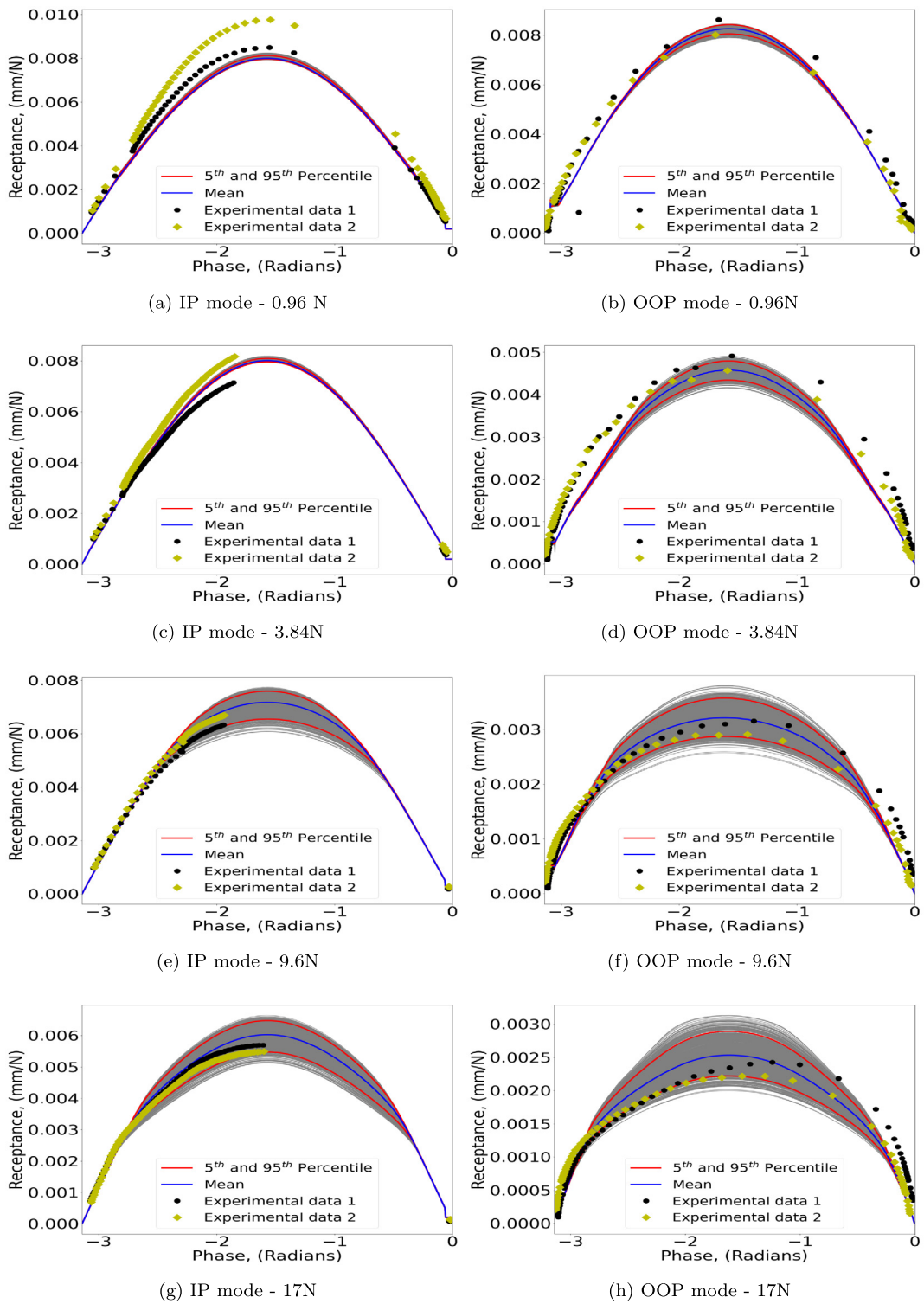
Fig. 11. Comparison of amplitude response from the updated PCE models and experimental data from the UPD rig.
