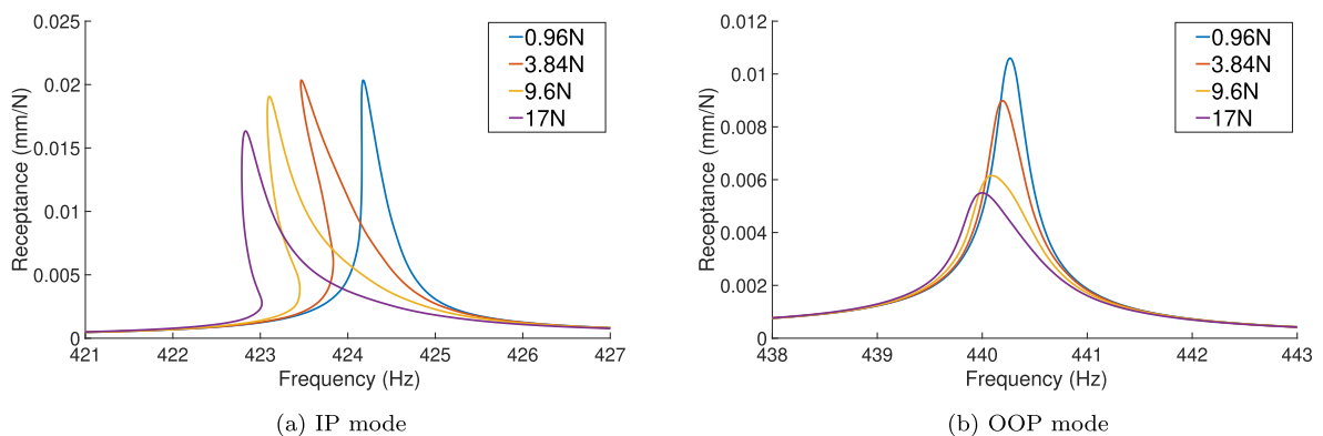
Fig. 3. Numerical simulations of the forced frequency response at different excitation levels.
