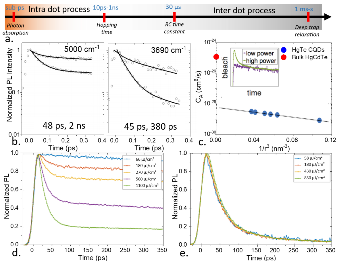
Figure 24 a. Time scale of the different carrier relaxation times in a film of HgTe NPLs b. PL decays for HgTe CQDs emitting at 2 \mu\text{m} (left) and 2.7 \mu\text{m} (right). The open circles denote the measured intensity; the solid lines represent the biexponential fits with the time constants presented as labels. The samples were excited with 1.2 mW (high power) and 0.027 mW (low power). Part b is adapted with permission from ref 168 Copyright (2014), American Chemical Society. c. Magnitude of the Auger coefficient as a function of the inverse of the particle volume for HgTe NCs. Part c is adapted with
