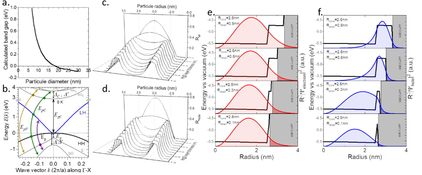
Figure 15 a. Prediction of the bandgap from the HgTe particle size using the effective mass approximation. Part a is used with permission from the Royal Society of Chemistry, from ref 93 ; permission conveyed through the Copyright Clearance Center. b. Simulated dispersion E_i(k) for the 14 bands of the k.p model. Part b is adapted with permission from ref 62 Copyright (2020) American Chemical Society. Radial wave functions of the electrons (c.) and holes (d.) in CdS/HgS/CdS heterostructures with various HgS thicknesses. Parts c and d are reprinted with permission from ref 125 Copyright (1994) by the American Physical Society. Conduction band (e.) and valence band profiles (f) and electron/hole density distribution in HgSe/HgTe heterostructures for various thicknesses of the HgTe shell. Parts e and f are adapted with permission from ref 120 Copyright (2018) American Chemical Society.
