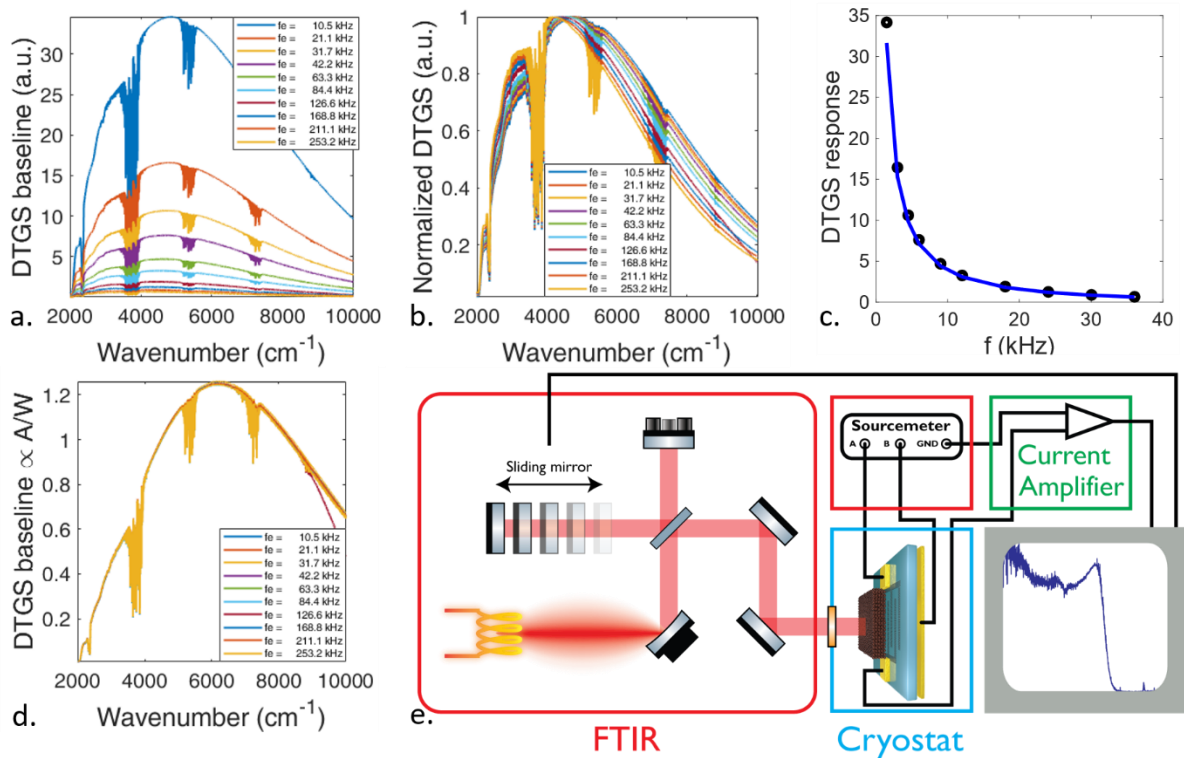
Figure 34 a. DTGS signal of an FTIR source measured at different sampling frequencies. b. Normalized DTGS signal at different sampling frequencies. c. Estimated transfer function at 4500\text{ cm}^{-1} and its fit by H(f) = (a + bf + cf^2 + df^3)^{-1} . d. DTGS source spectra at different sampling frequencies corrected by the transfer function. e. Scheme of a typical setup used to measure the spectral response. FTIR illuminates the sample that is biased by a source meter and can eventually be placed in a cryostat. The current is later amplified by a transimpedance amplifier and sent back to the FTIR electronics to compute the Fourier transform.
