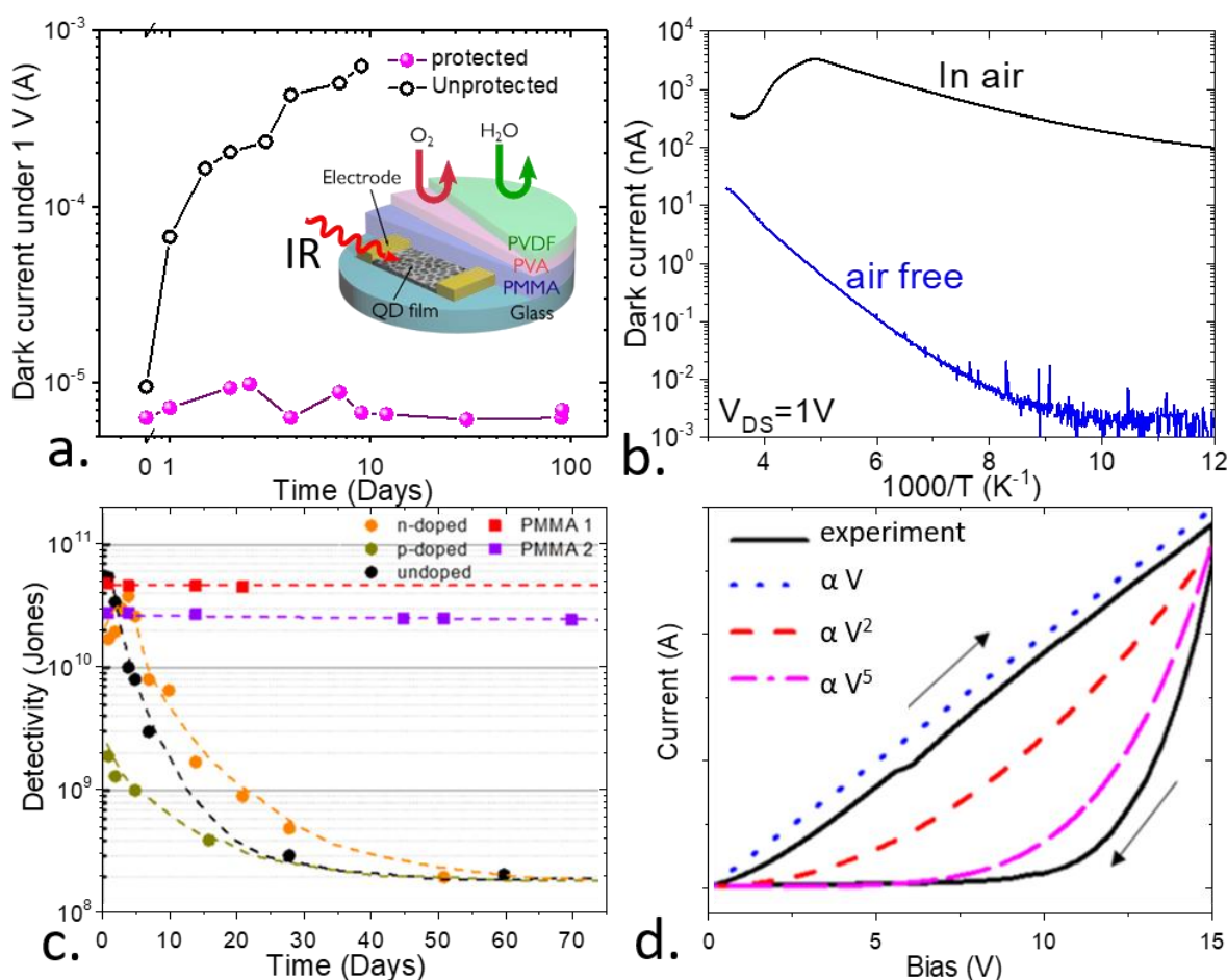
Figure 30 a. Dark current as a function of time spent in air for a HgTe CQD film with and without protective layers. Time zero corresponds to the sample in the air free glove box. The inset is a scheme of the HgTe CQD film device with polymer protective layers. Part a is adapted with permission from ref 302 Copyright (2018), American Chemical Society. b. Current as a function of temperature for a film of HgTe CQDs processed with ethanedithiol under air (black) and air free (blue) conditions. Part b is reprinted with permission from ref 35 . Copyright © 2013 WILEY-VCH Verlag GmbH & Co. KGaA, Weinheim c. Detectivity of photoconductive devices using a HgTe/hybrid with and without
