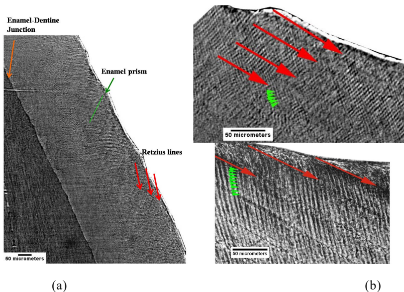
Figure 1: Reconstructed X-ray images of the sample Velia 387, cuspal portion of the upper deciduous central incisor showing the enamel microstructures (isotropic voxel size 1.3 \mu\text{m} ): (a) the Enamel-Dentine Junction, Retzius lines and enamel prism are highlighted; (b) upper panel, same as in (a) magnified, Retzius lines highlighted by red arrows, enamel prisms with daily cross striations pointed by green arrows; lower panel in (b) shows, for comparison, a histological thin section imaged in transmitted light microscopy.
