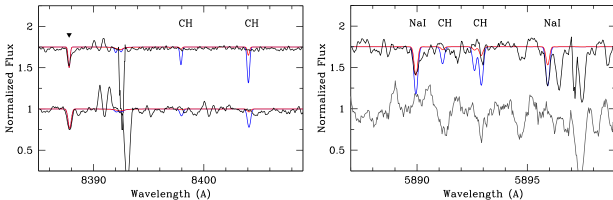
Figure 3. Left-hand panel: spectrum synthesis of the CH features near 8400 Å. Red syntheses indicate the best fits, where [\text{C}/\text{Fe}] = -1.0 . For illustration, a second fit for both spectra with [\text{C}/\text{Fe}] = 0.0 is shown in blue. The imperfect sky subtraction in the two-fibre mode GRACES spectra can be seen near 8392 Å. Right-hand panel: spectrum syntheses of the NaD lines and CH features near 5890 Å in Star40 (the SNR for Star46 is too low). The best fits to Star40, with [\text{C}/\text{Fe}] = -1.0 and [\text{Na}/\text{Fe}] = -1.4 is shown in red, and [\text{C}/\text{Fe}] = 0.0 and [\text{Na}/\text{Fe}] = -0.8 in blue. We take the average for sodium, thus [\text{Na}/\text{Fe}] = -1.1 \pm 0.3 . The imperfect sky subtraction in the two-fibre mode GRACES spectra can be seen near 5897 Å. In both panels, the spectral region for Star40 is offset by +0.75 in the flux for illustration.
