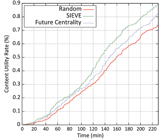
Fig. 5. Cumulative utility over time
