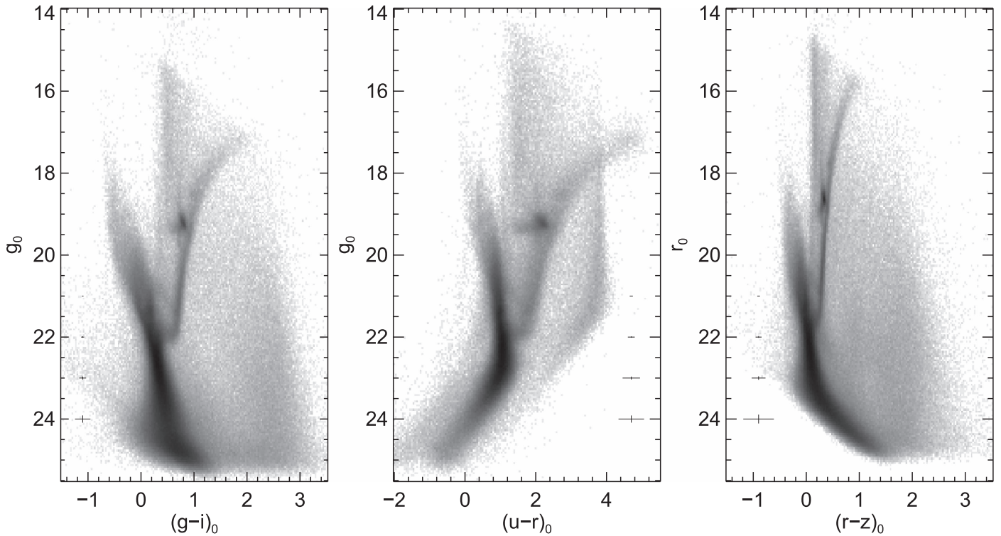
Figure 12. Multiple CMDs for Field55 using all ugriz bands. (Left) g_0 vs. (g-i)_0 , (middle) g_0 vs. (u-r)_0 , and (right) r_0 vs. (r-z)_0 . Error bars in magnitude and color are shown at the 21st, 22nd, 23rd, and 24th magnitude levels.
