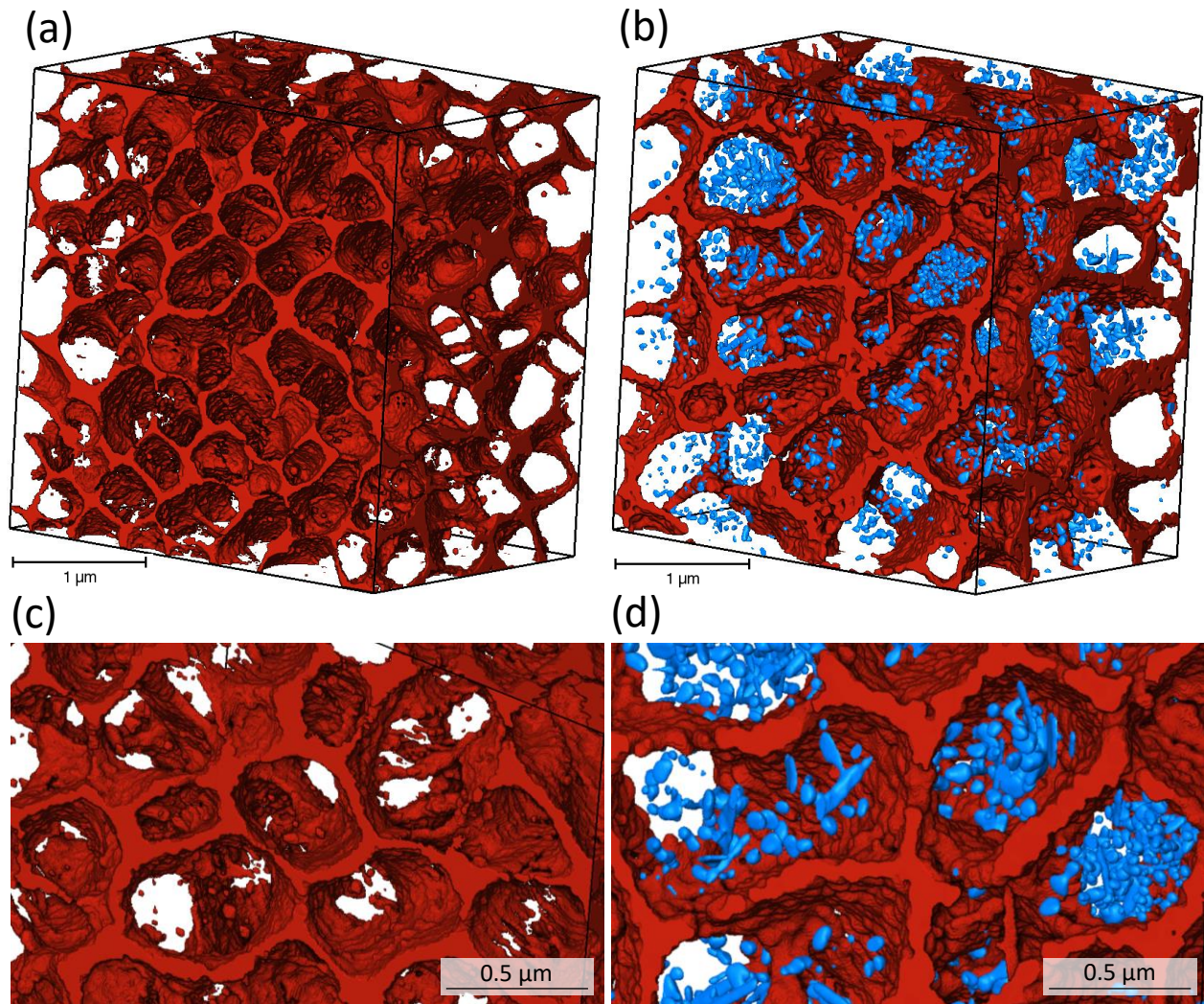
Fig. 8. FIB/SEM tomographies ( 3.5 \times 3.4 \times 2.5 \mu\text{m} ) of Si-rich phases of FMP zone of LPBF AlSi10Mg with building platform temperature of 35^\circ\text{C} (a) and 200^\circ\text{C} (b) and respective zoomed regions for detail (c,d).
