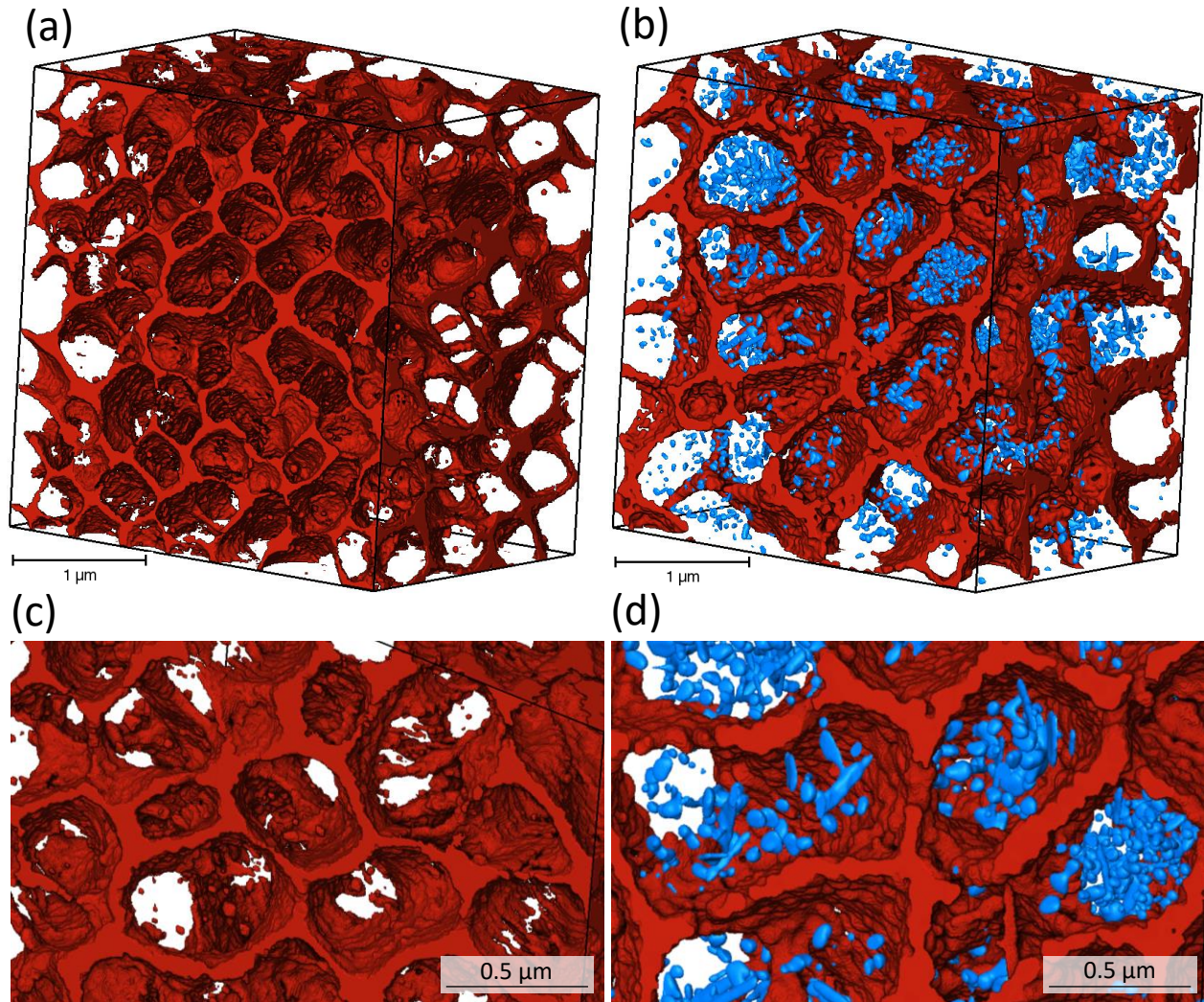
Fig. 8. FIB/SEM tomographies (3.5x3.4x2.5 µm) of Si-rich phases of FMP zone of LPBF AlSi10Mg with building platform temperature of 35°C (a) and 200°C (b) and respective zoomed regions for detail (c,d).
