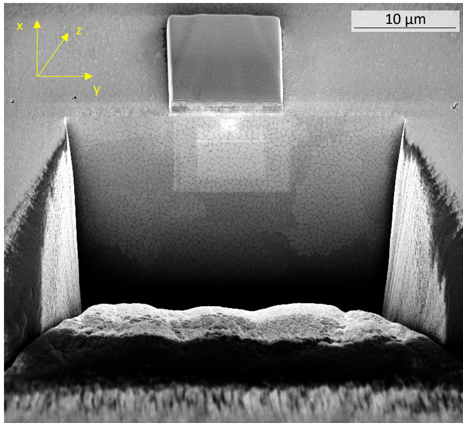
Fig. 3. Sample prepared for FIB/SEM tomography. The ion beam induced carbon coating can be observed on the top of the figure. The trench at the front of the figure is created by removing material by FIB to expose the surface that will be the section of the FIB/SEM tomography volume. The sample x, y, z orientation axis is in reference to Fig. 2.
