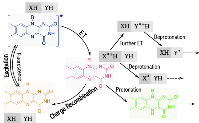
Figure 1. General reaction pathways for light-induced processes in flavoproteins. Flavin is represented by the isoalloxazine moiety. XH and YH stand for aromatic residues (tryptophan or tyrosine), for simplicity limited to two. Anion protonation and cation deprotonation may be coupled, corresponding to proton transfer from residue to flavin (not explicitly depicted). For simplicity back reactions beyond the primary radical pair are not shown.
