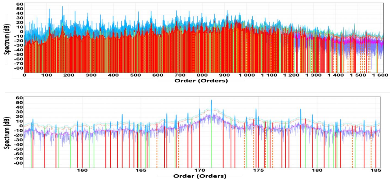
Figure 8. Two frequency zooms of an interpreted spectrum of a GOTIX vibration signal. The spectrum (purple) is estimated by a Welch method with Blackman window. The noise line (pink) is estimated by a nonlinear filter. Each detected peak has two colors: the upper color is related to its probability of false alarm (blue for high confidence, green for middle confidence and red for low confidence) and the lower color to its bandwidth (red for equivalence with the spectral window, green for a higher bandwidth, orange for a bad spectral window match).
