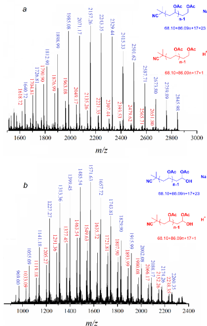
Figure 1. Polymer chain end group analysis using ESI spectra. a (Salen)Co III -PVAc ( M_{n,GPC} = 2.1 kDa, \mathcal{D} = 1.05 ). b The acidolysis product of (Salen)Co III -PVAc ( M_{n,GPC} = 1.8 kDa, \mathcal{D} = 1.07 ) in the presence of 3.0 MPa O 2 and acetic acid.
