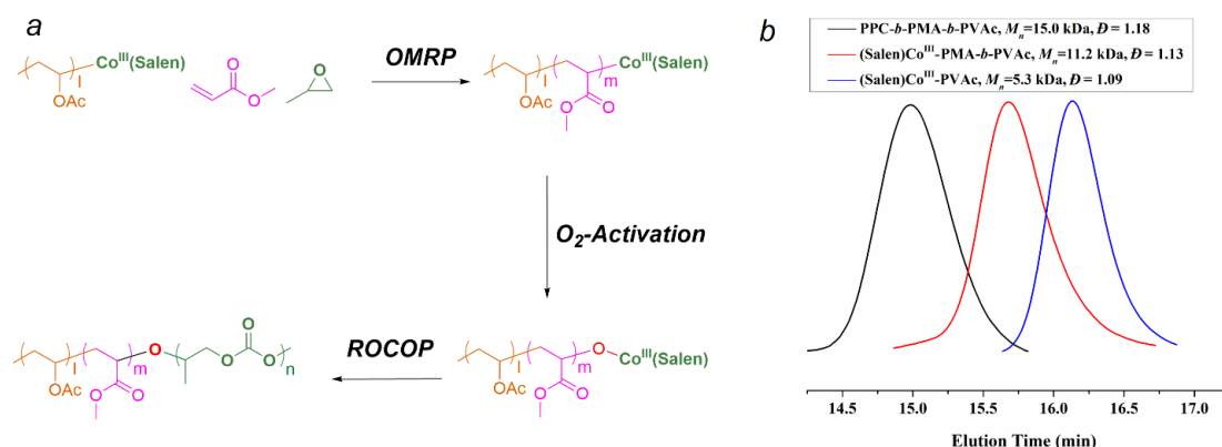
Figure 5. Synthesis of triblock copolymer. a Procedures for O_2 -triggered switchable polymerization from mixture of (\text{Salen})\text{Co}^{\text{III}}\text{-PVAc} macro-initiator, MA and PO under condition: [(\text{Salen})\text{Co}^{\text{III}}\text{-PVAc}]/[\text{MA}]/[\text{PO}] = 1/220/500 , OMRP of MA within 10 h at 60 °C, conv.=30%; O_2 -Activation within 12 h at 60 °C under 3.0 MPa O_2 , ROCOP of PO/ CO_2 within 8 h at 25 °C under 3.0 MPa CO_2 , conv.=7.5%. b GPC traces of the (\text{Salen})\text{Co}^{\text{III}}\text{-PVAc} macro-initiator, M_n = 5.5 kDa, \bar{D} = 1.09 ; (\text{Salen})\text{Co}^{\text{III}}\text{-PMA-}b\text{-PVAc} , M_n = 11.2 kDa, \bar{D} = 1.13 ; \text{PPC-}b\text{-PMA-}b\text{-PVAc} , M_n = 15.0 kDa, \bar{D} = 1.18 .
