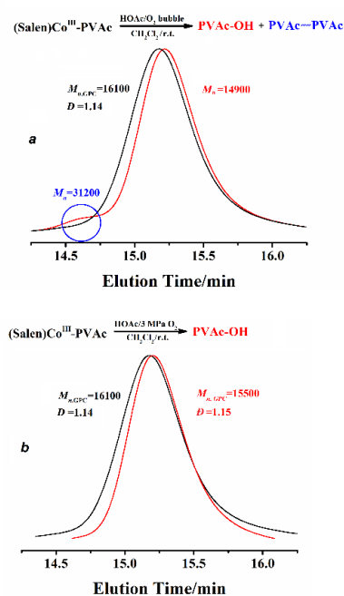
Figure 3. GPC curves of (Salen)Co III -PVAc ( M n,GPC = 16.1 kDa, D = 1.14) (black) and of the corresponding oxidation/acidolysis product (red). a Comparison of (Salen)Co III -PVA and the acidolysis product obtained with O 2 bubbling at atmospheric pressure. b Comparison of (Salen)Co III -PVA and the acidolysis product obtained under a high O 2 pressure (3.0 MPa).
