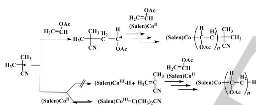
Figure 2. Plausible pathway for PVAc with cyanoisopropyl chain end group. Reactions of the cyanoisopropyl radical with (Salen)Co II and VAc.
