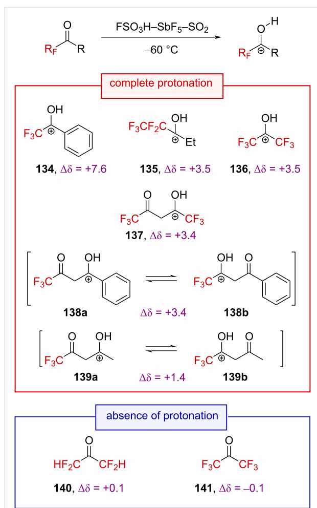
Scheme 34: Direct NMR observation of the protonation of some trifluoromethyl ketones in situ and the corresponding ^{19}\text{F} NMR chemical shifts. \Delta\delta = \delta_{^{19}\text{F,product}} - \delta_{^{19}\text{F,precursor}} ( \delta in ppm).
