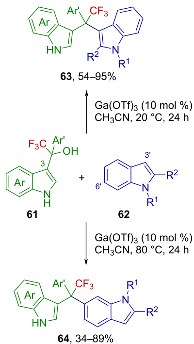
Scheme 17: \text{Ga}(\text{OTf})_3 -catalyzed synthesis of 3,3'- and 3,6'-bis(indolyl)methane from trifluoromethylated 3-indolylmethanols.
