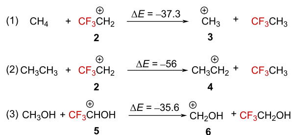
Scheme 1: Isodesmic equations accounting for the destabilizing effect of the \text{CF}_3 group. \Delta E in \text{kcal}\cdot\text{mol}^{-1} , calculated at the 4-31G level.
