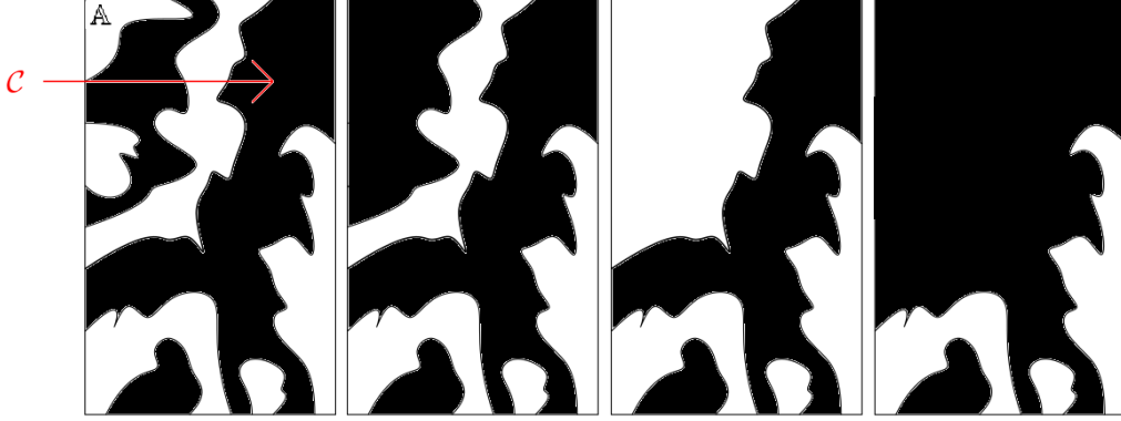
FIGURE 2. The final loop of the algorithm in the proof of the third statement of Lemma 3.6; this loop occurs when there is no left-right or top-bottom paths in \{f = 0\} \cap B_k(R) . In this example the loop expands the area \mathbb{A} three times in order to determine the sign \mathcal{C} of the crossing.
