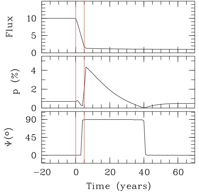
Fig. 2. STOKES simulation of a type 1 quasar that suffers dimming of the continuum source by a factor of 10 in 5 years (indicated by the red vertical lines). Top: total flux in arbitrary units seen by the observer as a function of time. Middle: evolution of the polarization degree ( p in percent). Bottom: evolution of the polarization position angle ( \Psi in degrees).
