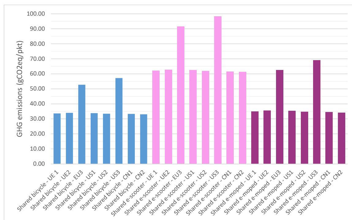
Figure 6 Carbon footprint of the shared modes depending on shipping type
