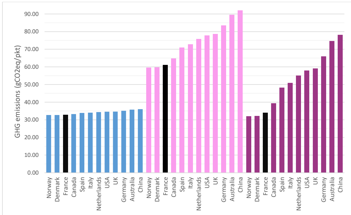
2 Figure 7 Carbon footprint of the shared modes depending on the electricity mix: shared bikes in 3 blue, shared ES in pink, shared e-mopeds in purple, and French reference in black
