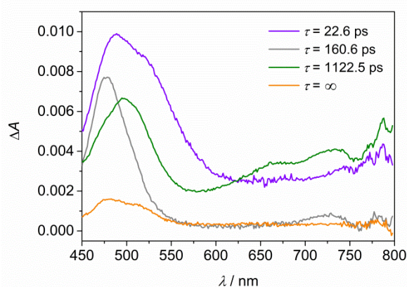
Figure 4. a) Transient absorption spectra of Rot 1s -PTZ in CH 3 CN measured at the end of pulse and at various delays. b) Spectral distribution of the amplitudes of the calculated lifetimes (indicated in the legend) from global fit analysis of the transient absorption matrix (obtained with four principal components and three expected lifetimes, plus an infinite lifetime). \lambda_{exc} = 350 nm ( A_{350} = 0.2 , 2 mm optical path).
