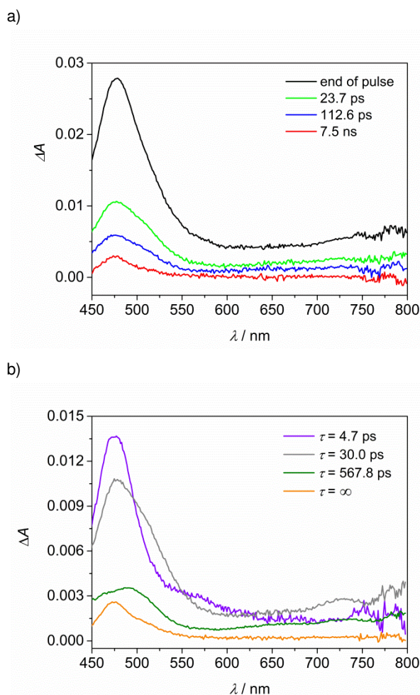
Figure 5. a) Transient absorption spectra of Rot' 2s -PTZ in CH 3 CN measured at the end of pulse and at various delays. b) Spectral distribution of the amplitudes of the calculated lifetimes (indicated in the legend) from global fit analysis of the transient absorption matrix (obtained with four principal components and three expected lifetimes, plus an infinite lifetime). \lambda_{\text{exc}} = 350 nm ( A_{350} = 0.2 , 2 mm optical path).
