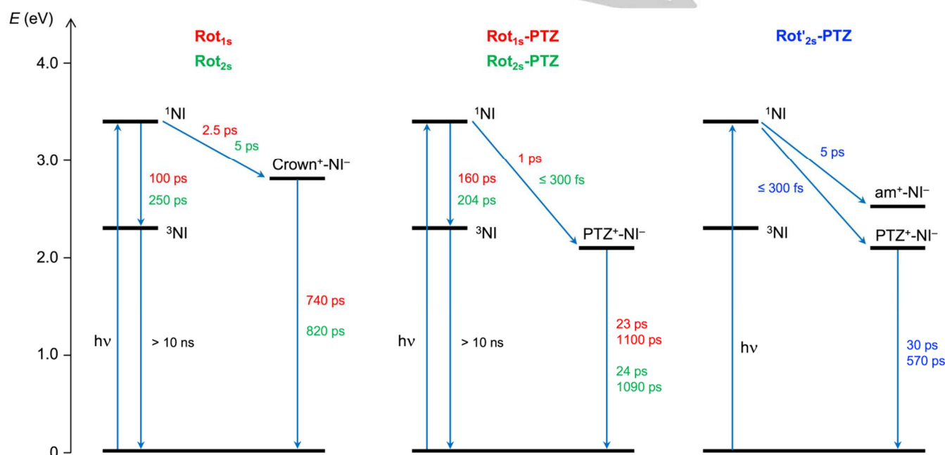
Figure 6. Simplified energy-level diagram with a schematic representation of the main photophysical processes that occur in the different rotaxanes. The different arrows departing from the same 1 NI excited state denote processes that occur in different conformations of the rotaxane and are not competitive processes that can occur in the same conformation. The reported lifetimes are those measured by transient absorption spectroscopy (from global analysis, in particular, when performed; see the text). The energy values of the NI-localized singlet and triplet excited states have been taken from the literature, [31] while those of the charge-separated states have been estimated from redox potentials determined in this work or reported in the literature. [14]
