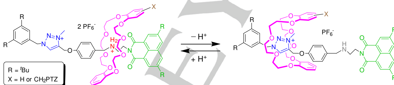
Scheme 1. The acid-base triggered rearrangement of the rotaxanes studied in this work. Two selected conformations for the flexible ring are represented to emphasize the fact that shuttling does not necessarily result in a net modification of the distance between A (naphthalimide stopper) and D [phenothiazine (PTZ) unit appended to the DB24C8 macrocycle]. Other ring conformations and relative ring-axle orientations are possible for both states.
