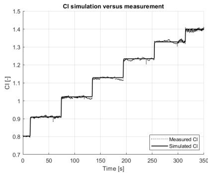
Fig. 14: C_L simulation versus measurement.
