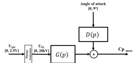
Fig. 7: System diagram.
