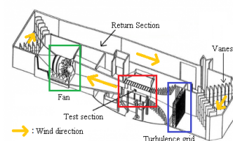
Fig. 1: Large subsonic wind tunnel diagram (PRISME Laboratory).
