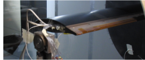
Fig. 3: Picture of the bidimensional configuration of the blade.
