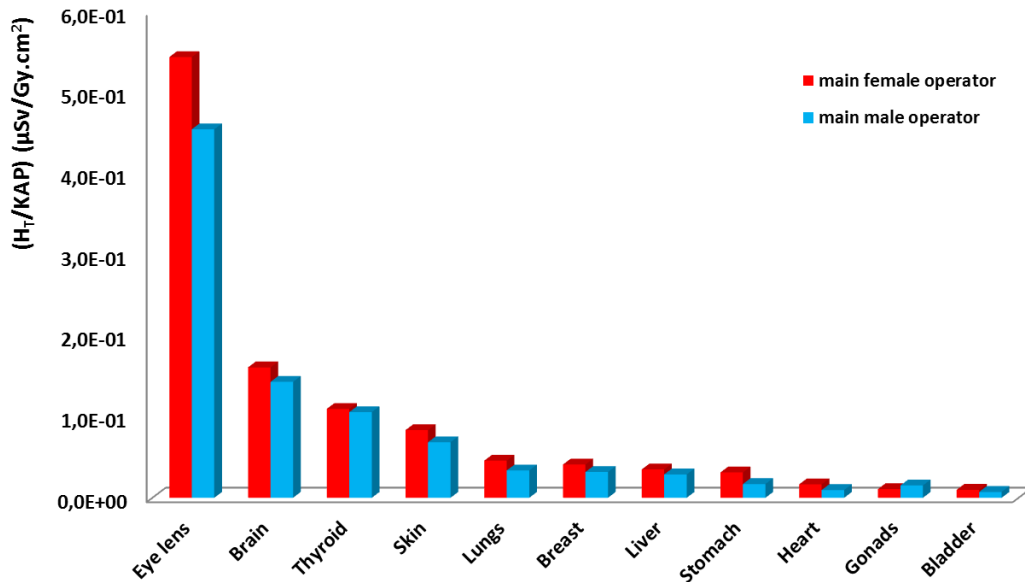
Figure 8. Comparison of equivalent dose ( H_T/KAP ) for some organs of the main male and female operators, for RAO25^\circ projection ( kVp=100\text{ kVp} , FOV=20 \times 20\text{ cm}^2 ).
