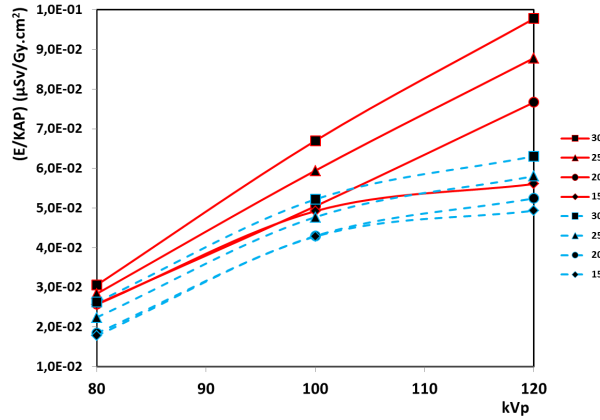
Figure 4. Occupational effective dose function of kVp for different FOV: 15 \times 15 \text{ cm}^2 / 20 \times 20 \text{ cm}^2 / 25 \times 25 \text{ cm}^2 / 30 \times 30 \text{ cm}^2 (continuous: main operator, discontinuous: assistant operator).
