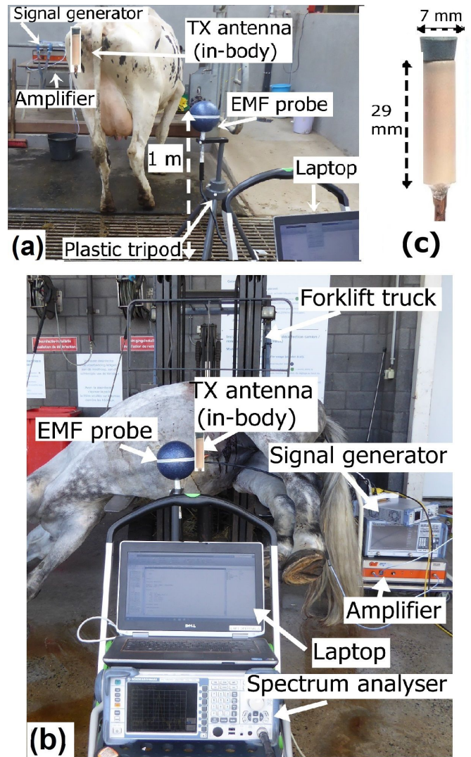
Fig. 1. Setup for the (a) cow and (b) horse measurements. (c) The capsule antenna after the preparation for the measurements (see [30] for more details).
