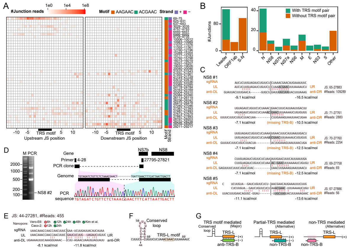
Figure 4: TRS motif independent RNA-RNA interaction in template switch
