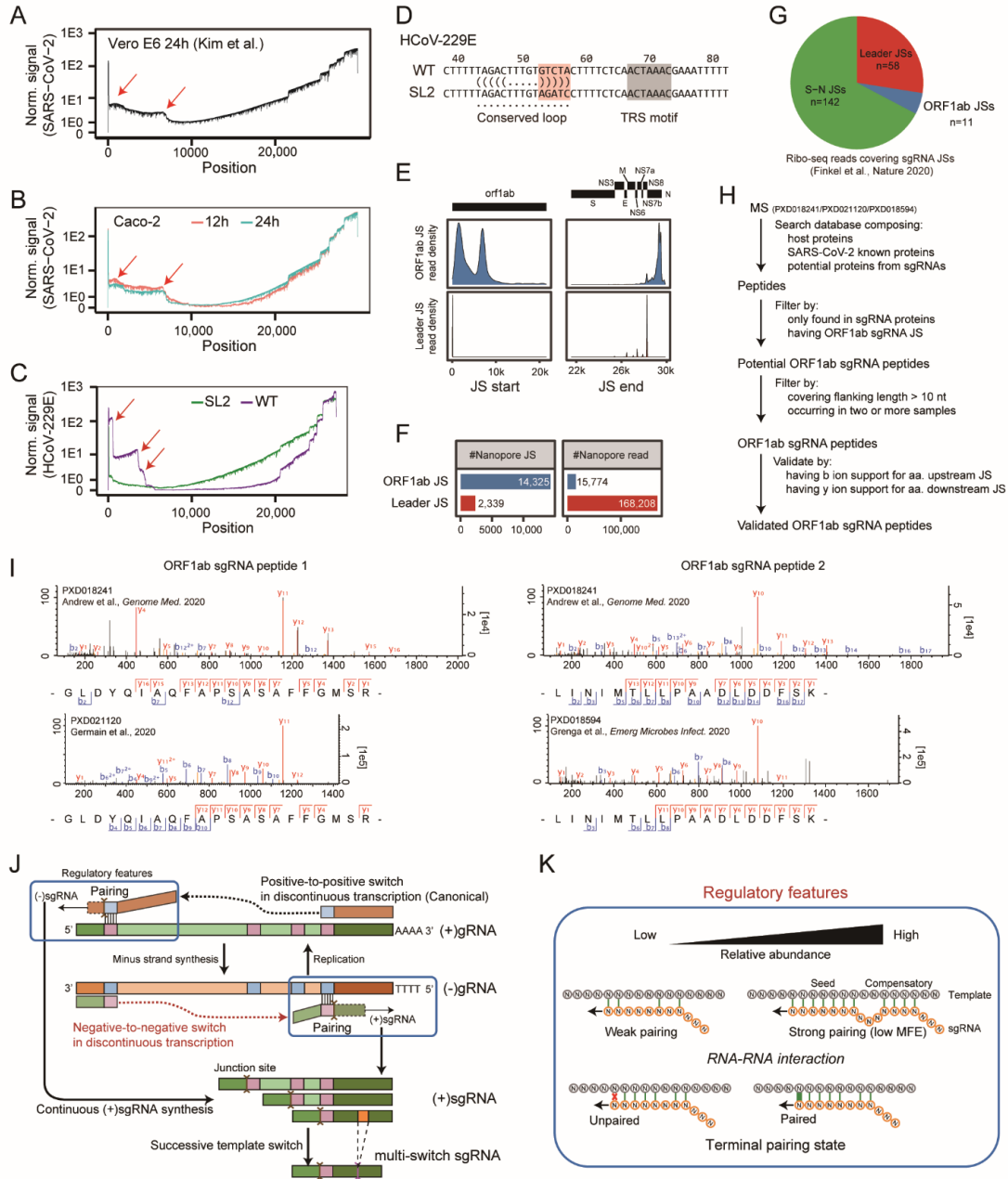
Figure S7: Non-canonical template switches in different coronaviruses, related to Figure 5 (A) Nanopore read coverage profile across the SARS-CoV-2 genome post-infection in Vero E6 cells from the Kim et al. study. The arrows in ORF1ab region mark obvious loci with abrupt changes indicating template switch junctions. (B) Nanopore read coverage profiles across the SARS-CoV-2 genome in Caco-2 cells at 12 h and 24 h post-infection. (C) Nanopore read coverage profiles across the HCoV-229E genome for WT and SL2 strains 24 h post-infection in Huh7 cells from the Viehweger et al. study. (D) Sequence difference between the WT and SL2 strain for HCoV-229E virus. (E) The distribution of junction boundaries (left for JS start and right for JS end) from Nanopore data for ORF1ab-mediated (top) and Leader sequence-mediated (canonical, bottom) long-range template switches in Vero E6 cells 48 h post SARS-CoV-2 infection. (F) The number of different junction sites (JS, left) and reads (right) for ORF1ab-mediated and Leader sequence-mediated (canonical) template switches supported by Nanopore data from Vero E6 cells 48 h post SARS-CoV-2 infection. (G) Statistics of different types of junction sites (JSs) covered by SARS-CoV-2 Ribo-seq reads from the Finkel et al. study. (H) Mass Spectrometry (MS) data processing pipeline to identify sgRNA derived peptides. (I) Mass spectrum of the ORF1ab-type peptides in Figure 5G with both y and b ion supports. (J) Graphical illustration for positive-to- positive (canonical) and negative-to-negative switching modes in generating single- and multi- switch sgRNAs from discontinuous transcription from gRNA. (K) Graphical illustration of regulatory features in governing sgRNA abundance. Strong RNA-RNA base-pairings (low MFE, Minimum Free Energy of base-pairings) and terminal pairing status would lead to efficient template switching and high abundance of corresponding sgRNA.
