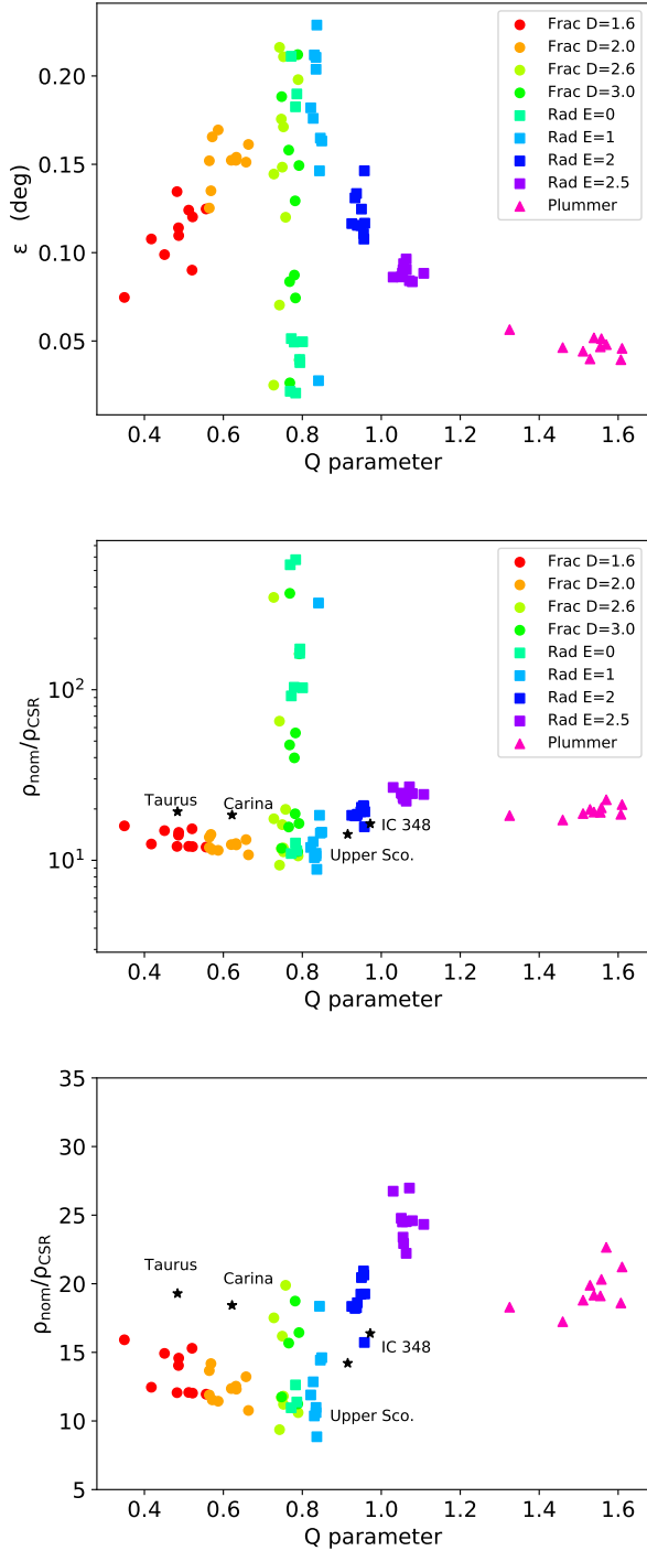
Fig. 4. Top: \epsilon scale parameter for DBSCAN calculated with the procedure presented in Sect. 2.2 against Q structure parameter. Middle: relative nominal density of the detected structures ( \frac{\rho_{\text{nom}}}{\rho_{\text{CSR}}} , as described in the text) against Q structure parameter. Colours and symbols represent parent distributions, with the same code as in Fig. 3. Bottom: same plot as in the middle panel, linearly scaled and zoomed, so that the general trends are clearer.
