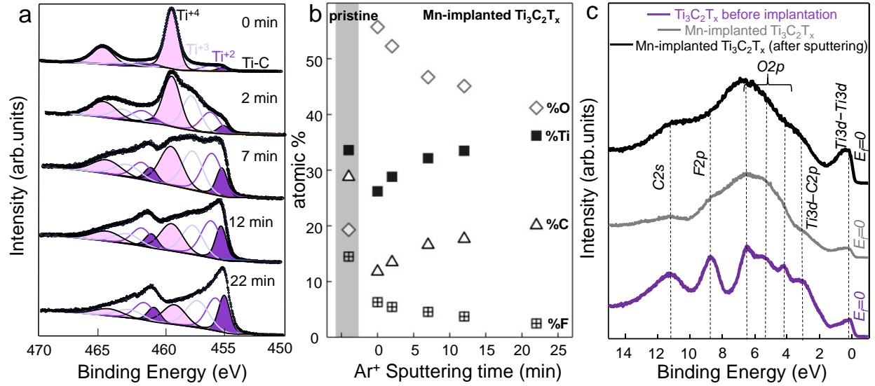
Figure 3. a) Ti2p HR-XPS spectra of \text{Mn}^{+} -implanted \text{Ti}_3\text{C}_2\text{T}_x thin film ( 1 \cdot 10^{15} ions/ \text{cm}^2 at 60 keV) after sputtering at different times; b) Evolution of the film composition (O, Ti, C, and F atomic %) with the sputtering time (500 eV \text{Ar}^+ ) as derived from the analysis of survey spectra for the Mn-implanted film as compared to the pristine \text{Ti}_3\text{C}_2\text{T}_x film (before implantation); c) Valence band XPS spectra of pristine \text{Ti}_3\text{C}_2\text{T}_x thin film, after implantation with 1 \cdot 10^{15} ions/ \text{cm}^2 at 60 keV, and after 22 min \text{Ar}^+ ion beam etching.
