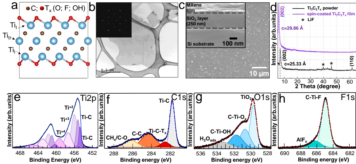
Figure 1. MXenes powder and thin film characterization. a) The schematic structure 60 of monolayer \text{Ti}_3\text{C}_2\text{T}_x MXene; \text{Ti}_\text{I} and \text{Ti}_\text{II} are surface and core Ti atoms, respectively, T is a surface functional group; b) TEM micrograph of \text{Ti}_3\text{C}_2\text{T}_x flakes obtained from a delaminated colloidal MXene solution with corresponding SAED pattern (inset); c) SEM image of MXene spin-coated thin film with a corresponding cross-section (inset) taken in Secondary Electron Imaging (SEI)
