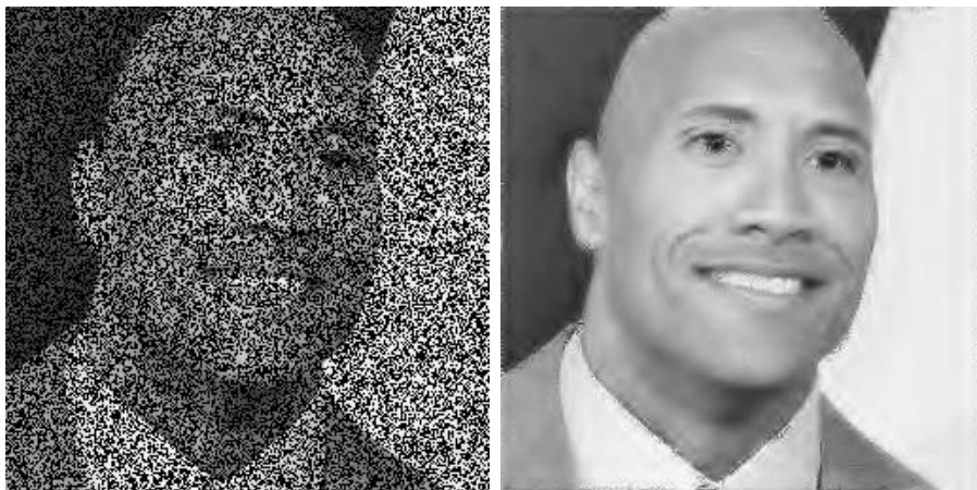
Figure 3: Example of image inpainting: the damaged image y is on the left and an approximation of the solution of (38) is on the right.
