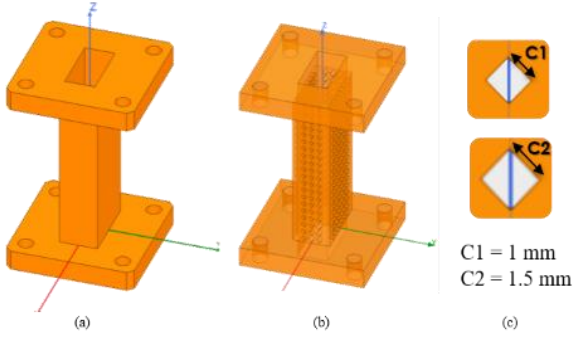
Fig. 1. Structural illustration of Ku-band waveguides designed on HFSS TM . (a) Full-metal waveguide. (b) Perforated waveguide with C1=1 mm. (c) Shape of cubic grids for both perforated waveguides.
