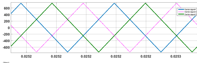
Fig. 2. Shifted carriers
