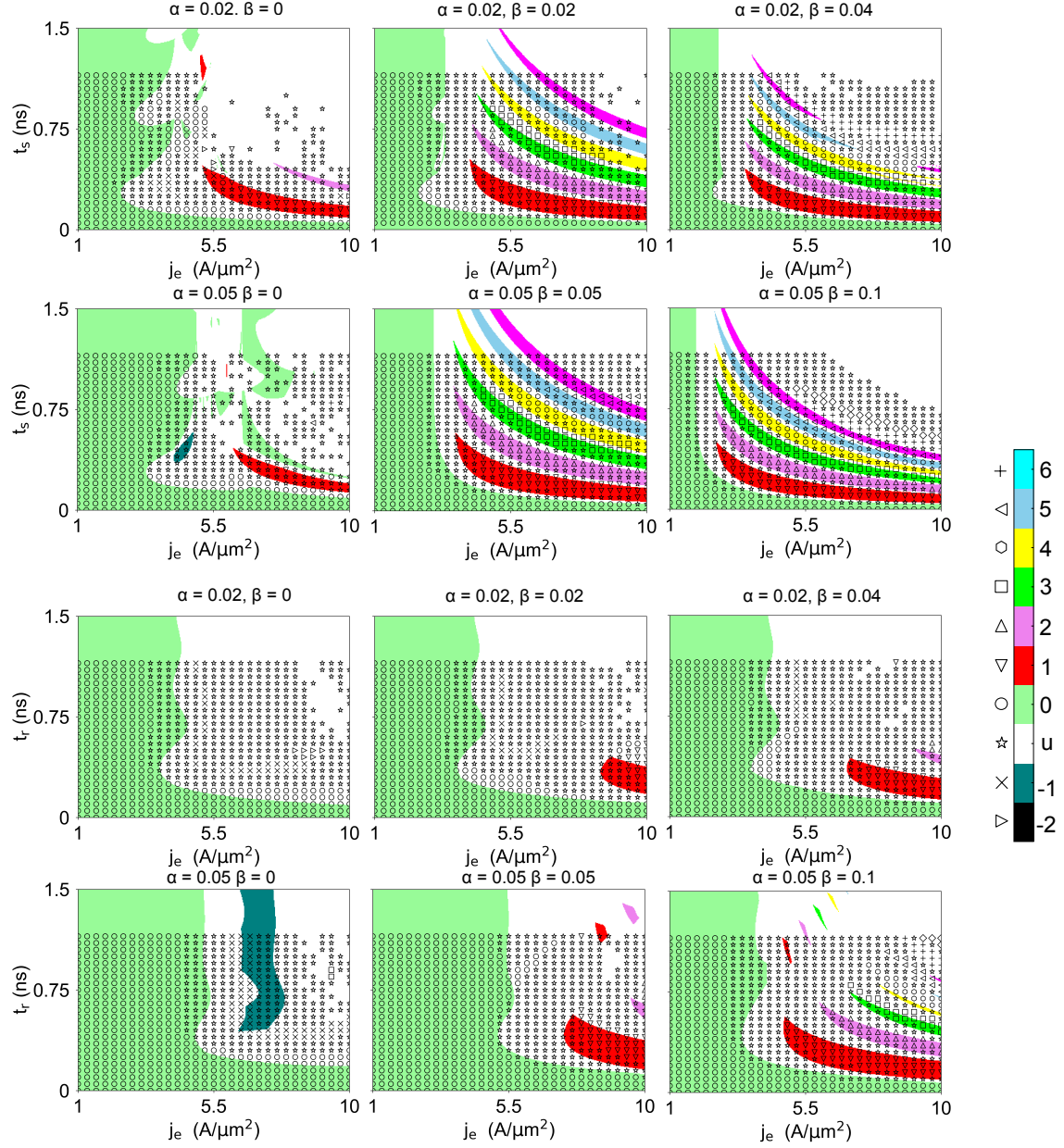
FIG. S2. (Color online) Phase diagrams of a train of two DWs situated at neighboring pinning centers, for different pulse and material parameters. The analytical calculation with the Heisenberg DW exchange interaction (colors) is superposed on the micromagnetic calculations (symbols).
