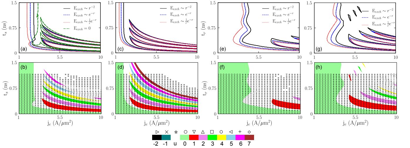
FIG. 2: (Color online). Contour plots of the different bands obtained for a train of two neighboring DWs with different type of DW exchange interaction at T=0\text{K} using the 1D model are represented in the upper panels (a), (c), (e) and (g). In the lower panels, the 1D results (colored regions) obtained for a Heisenberg type DW exchange interaction are compared with the micromagnetic calculations (scattered symbols) for the same pulse characteristics and \alpha and \beta parameters as the upper panels. The numbering of the bands is as follows: positive bands correspond to the DWs moving collectively in the direction of the electron flow with the same initial relative distance between them, negative numbers to the DWs moving collectively in the opposing direction with the same initial relative distance between them, zero state correspond to the DWs staying pinned at initial positions and 'u' to the unintended states in which the DWs do not move synchronously in either direction. The parameters used are: (a) and (b) t_s variable, t_r=t_f=5\text{ps} , \alpha=0.02 , \beta=0.04 , (c) and (d) t_s variable, t_r=t_f=5\text{ps} , \alpha=0.05 , \beta=0.1 , (e) and (f) t_r variable, t_s=t_f=5\text{ps} , \alpha=0.02 , \beta=0.04 , (g) and (h) t_r variable, t_s=t_f=5\text{ps} , \alpha=0.05 , \beta=0.1 .
