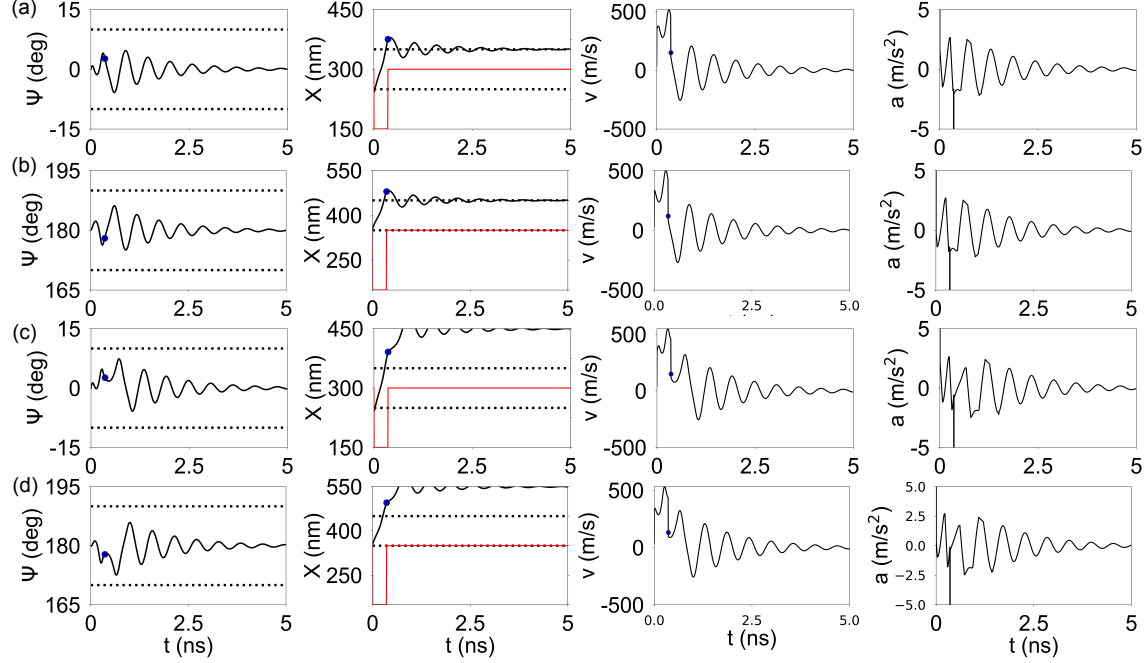
FIG. S4. (Color online) DW angular variation, position, velocity and acceleration for the first DW in (a) and (c) and second DW in (b) and (d) from a train of two neighboring DWs computed with the same pulse characteristics for a Heisenberg type DW exchange (a) and (b) and Yukawa-Reid type DW exchange in (c) and (d). The pulse parameters are: t_r = t_f = 5 ps, t_s = 350 ps and j_e = -4 A/ \mu\text{m}^2 which correspond to a +1 state with \alpha = 0.02 and \beta = 2\alpha . The Yukawa-Reid DW exchange gives a +2 state after one pulse, but an unintended state after several periodic pulses. The dotted lines in the angular variation panels represent the \pm 10^\circ around the equilibrium value, while in the position panels the dotted lines represent the position of the pinning centers in the nanowire. The current pulse shape is superimposed on the position panels. The dot represents the end of the pulse.
