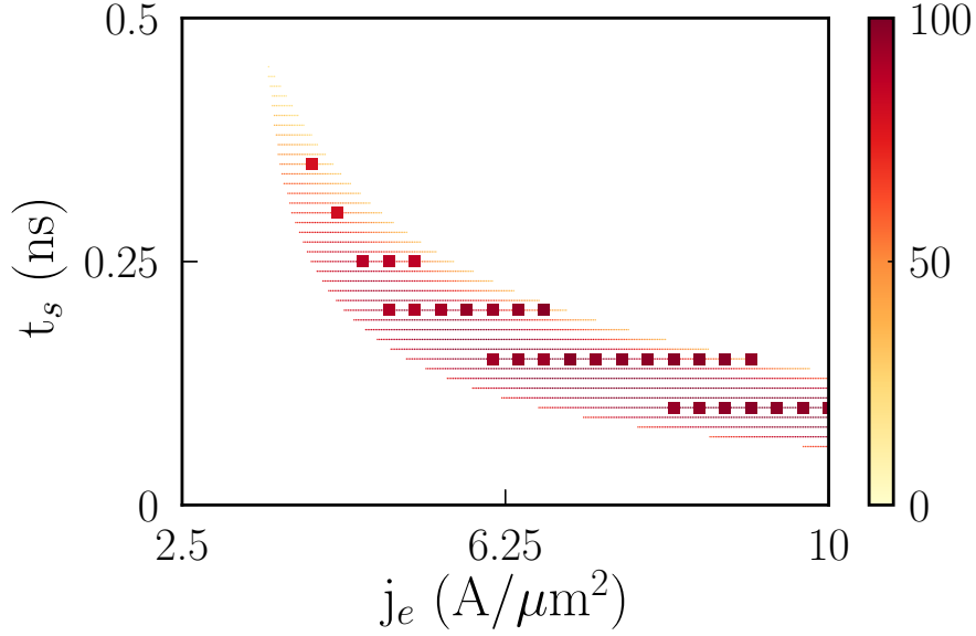
FIG. S5. (Color online) Probability of DWs motion in the +1 band for a train of two neighboring DWs at T=293\text{K} . The damping parameter is \alpha = 0.02 and \beta = 2\alpha . The micromagnetic results on 30 band points (large squares) are superposed on the analytical results on 3093 band points (small points - almost continuous).
