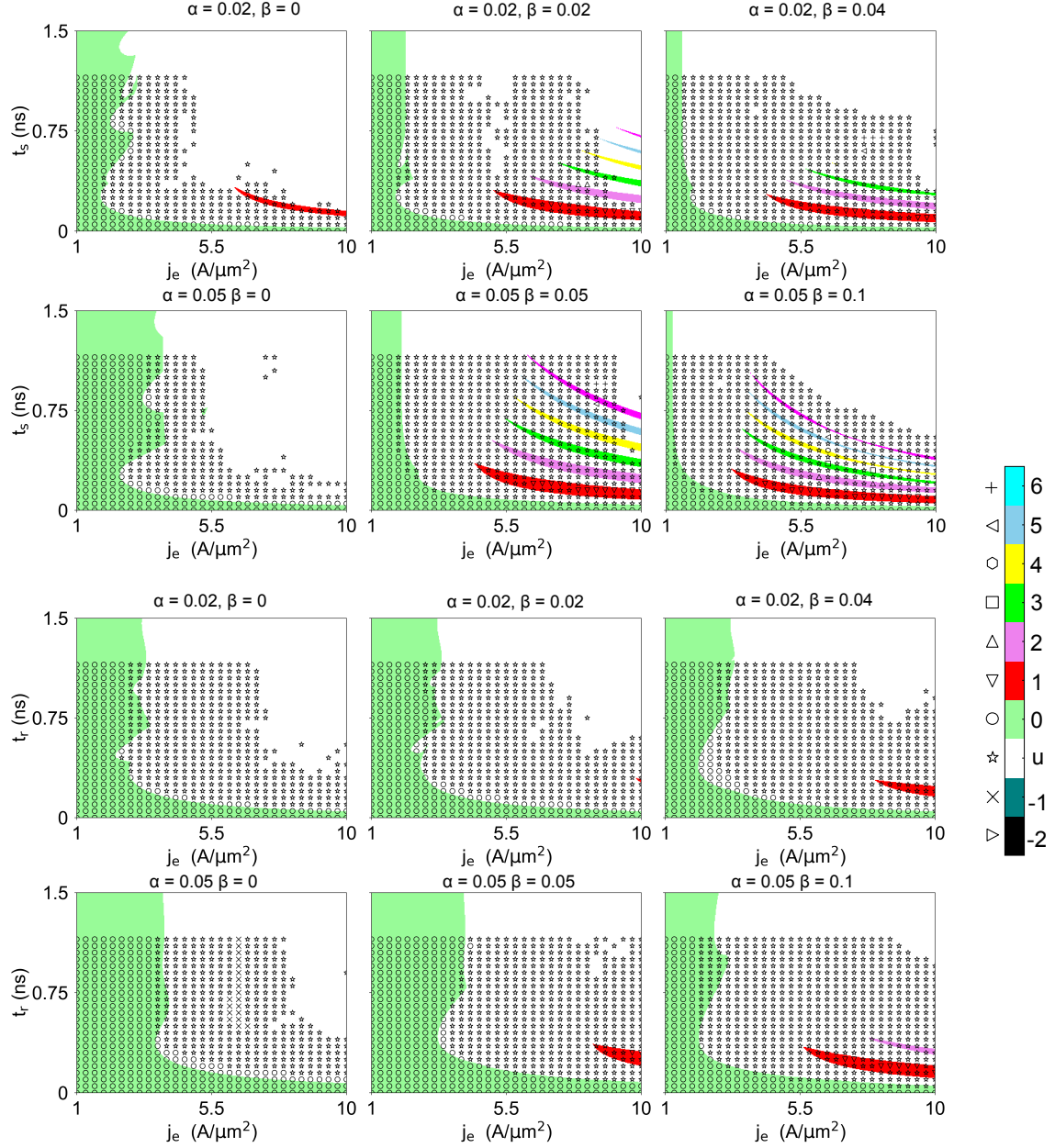
FIG. S3. (Color online) Phase diagrams of a train of four DWs situated at neighboring pinning centers, for different pulse and material parameters. The analytical calculation with the Heisenberg DW exchange interaction (colors) is superposed on the micromagnetic calculations (symbols).
