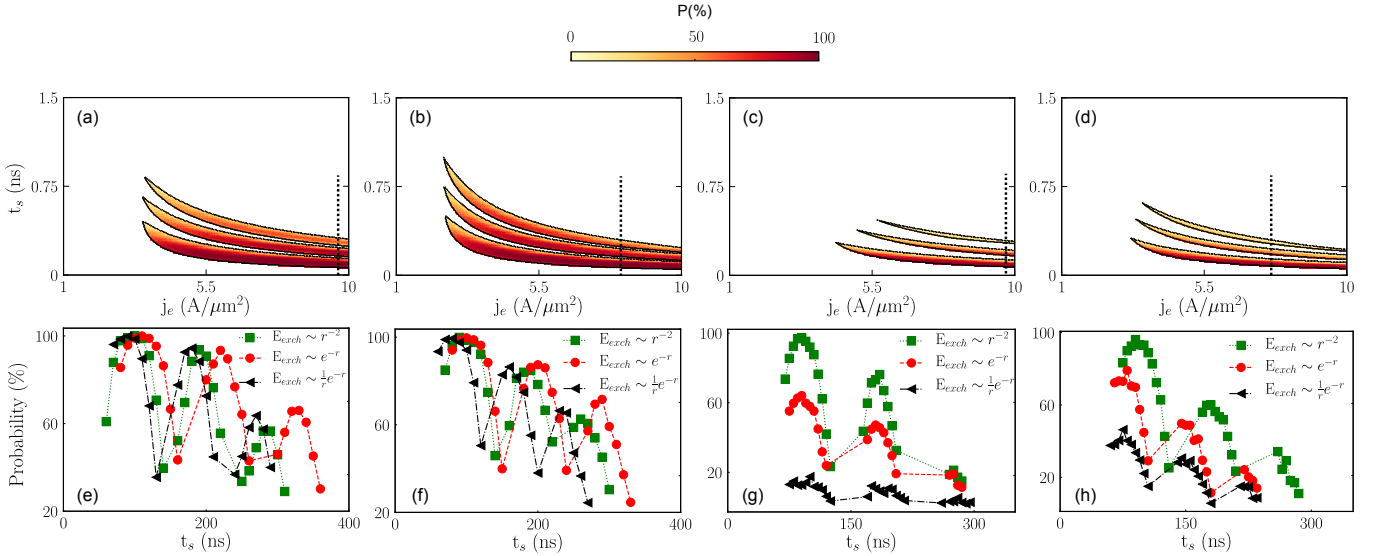
FIG. 5: (Color online) Probability of DWs motion in different bands at T=293\text{K} , for a train of two neighboring DWs and a damping parameter \alpha = 0.02 in (a) or \alpha = 0.05 in (b), or a train of four neighboring DWs with \alpha = 0.02 in (c) or \alpha = 0.05 in (d). A Heisenberg-type DW exchange interaction is used along with a non adiabatic parameter \beta = 2\alpha . The vertical dotted lines correspond to the probability profile represented in the figures underneath. The profiles are compared for different types of DW exchange interaction, and are chosen in each case as to pass through the maximum probability of the first band (the lowest branch in the figures).
