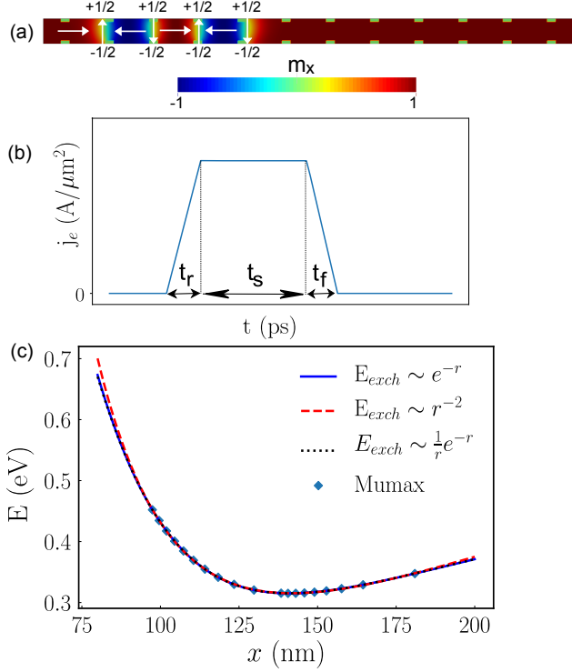
FIG. 1: (Color online) (a) Simulated structure with four magnetic domain walls with same topological charge are pinned at symmetric notches: two head-to-head and two tail-to-tail DWs. The fractional winding numbers of the edge defects are indicated for each DW. (b) Current pulse shape used to displace the domain walls. (c) Interaction energy of two domain walls in a nanowire without notches (symbols) as determined from micromagnetic simulations. The curves represent modeling with different trial functions.
