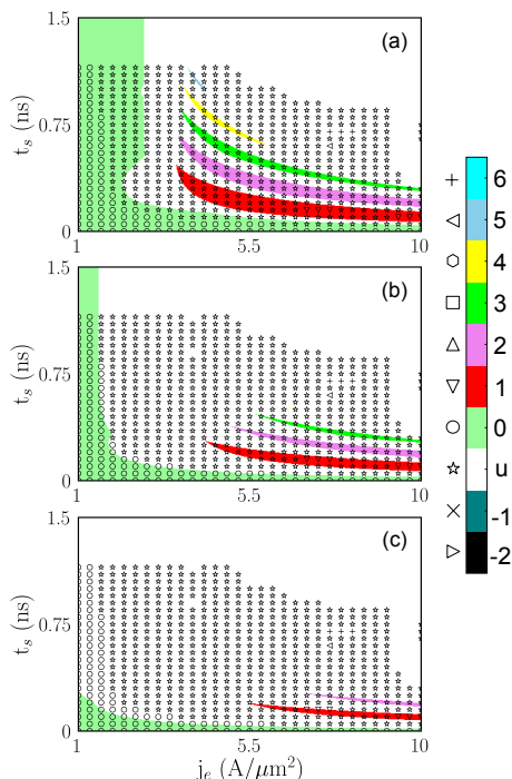
FIG. 3: (Color online) Influence of the Heisenberg DW exchange energy magnitude on the bands for a train of four neighboring DWs for \alpha=0.02 and \beta=0.04 : (a) a_1 = 0\text{eV} (no DW exchange), (b) a_1 = 1.0\text{eV} and (c) a_1 = 1.4\text{eV} . The 1D results (colored regions) obtained for a Heisenberg type DW exchange interaction are compared with the micromagnetic calculations (scattered symbols) at T=0\text{K} . The pulse stable time was varied, with t_r=t_f=5\text{ps} and t_z=10\text{ns} .
