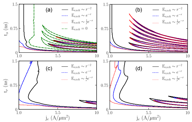
FIG. 4: (Color online) Contour plots of the different bands obtained for a train of four neighboring DWs (separated by 80\text{nm} ) with different type of DW exchange interaction at T=0\text{K} using the 1D model: (a) and (c) \alpha=0.02 and \beta=0.04 , (b) and (d) \alpha=0.05 and \beta=0.1 . In (a) and (b) the pulse stable time was varied, with t_r=t_f=5\text{ps} , while in (c) and (d) the raise time was varied with t_s=t_f=5\text{ps} and t_z=10\text{ns} .
