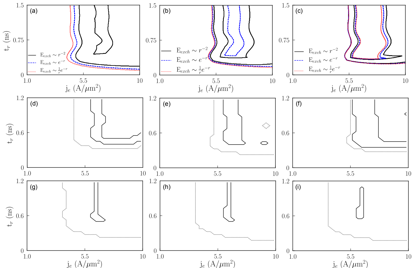
FIG. 6: (Color online) Influence of the pulse raise time t_r on the phase diagram for a train of several DWs at T=0K for \alpha = 0.05 and \beta = 0 . The parameter space is the raise time vs. current amplitude. In all cases, t_s = t_f = 5 ps and t_z = 10 ns. The 1D model results for different DW exchange energies are shown in panels (a) to (c) for a train of 2DWs separated by: (a) 80nm, (b) 160nm and (c) 240nm. Only the band -1 is visible in the center of the diagram, together with the depinning boundary. The micromagnetic results are presented in the panels (d) to (i), where the band -1 is represented by a continuous line and the limit of the band 0 by the dotted line. The micromagnetic simulations are for a train of two DWs separated by: (d) 80nm, (e) 160nm and (f) 240nm and a train of (g) three DW, (h) four DW and (i) five DW separated by 80 nm.
