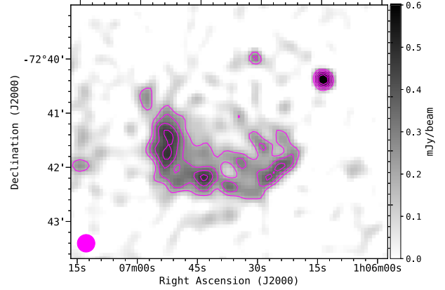
Figure 13. ASKAP ESP image of the new low surface brightness SMC SNR candidate MCSNR J0106–7242 at 1320 MHz (grey scale and contours) smoothed to a resolution of 20 \times 20 arcsec. Magenta contours are: 0.18, 0.27, 0.36, 0.45, and 0.54 mJy beam –1 . The smoothed beam is shown as a filled magenta circle in the lower left corner. The point-like source in the upper right corner is an unrelated background source. The local RMS noise is 0.06 mJy beam –1 .
