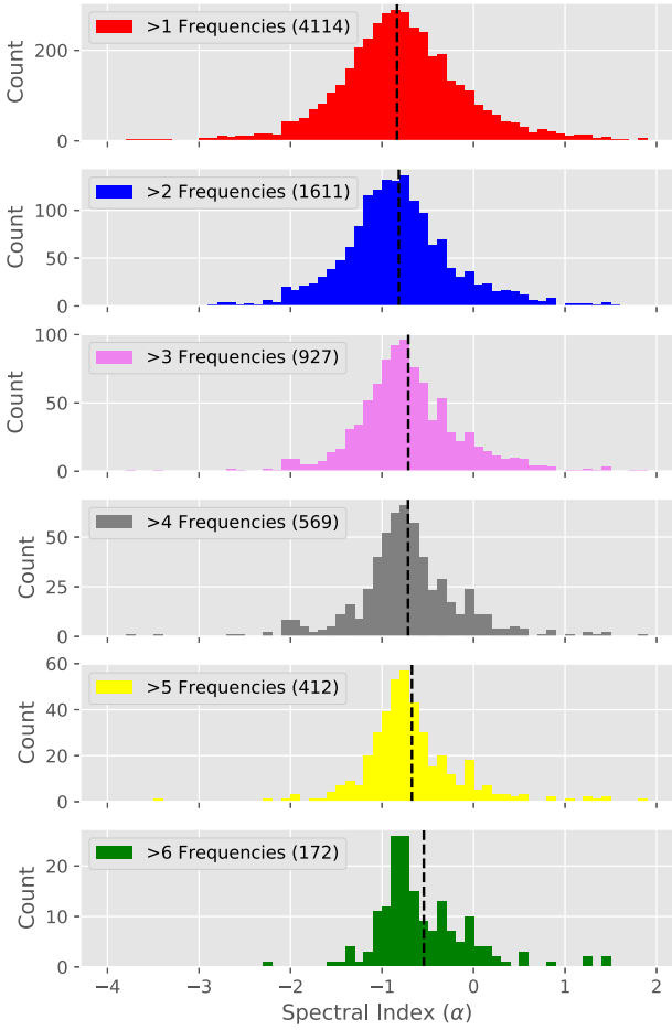
Figure 11. Spectral index distribution of all sources in the field of SMC binned at 0.1. The vertical dashed line represents the mean \alpha of each panel, as discussed in Section 3.3. The uppermost panel includes all the sources of the other panels beneath.
