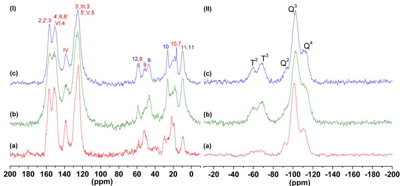
Figure 2. ^{13}\text{C}\{^1\text{H}\} CP MAS NMR (I) and ^{29}\text{Si}\{^1\text{H}\} CP MAS NMR spectra (II) of (a) \text{SiO}_2\text{-Ru} , (b) \text{SiO}_2\text{-RuYb} and (c) \text{SiO}_2\text{-RuNd} . 12: carbon atoms in methoxysilyl groups not grafted (Described the numbers in red and blue).
