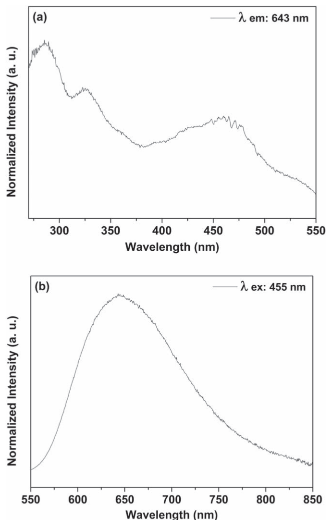
Figure 8. Room temperature excitation ((a), \lambda_{\text{emission}} = 643 \text{ nm} ) and emission ((b), \lambda_{\text{excitation}} = 455 \text{ nm} ) spectra of the \text{SiO}_2 Ru nanohybrid in solid state.
