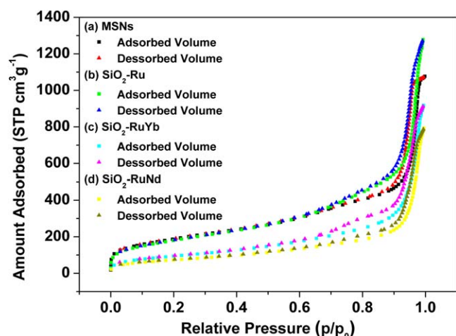
Figure 3. Nitrogen adsorption/desorption isotherms of (a) MSNs and (b) \text{SiO}_2\text{-Ru} , (c) \text{SiO}_2\text{-RuYb} and (d) \text{SiO}_2\text{-RuNd} nanohybrids.
