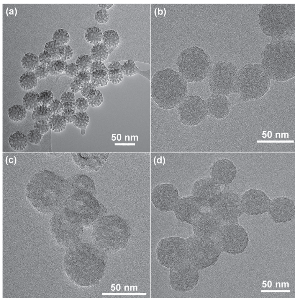
Figure 4. HR TEM images of (a) MSNs and different nanohybrids: (b) \text{SiO}_2 -Ru, (c) \text{SiO}_2 -RuYb and (d) \text{SiO}_2 -RuNd.
