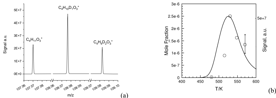
Fig. 5. (a) Mass spectrum showing the formation of C_4H_{10}DO_3^+ (m/z 108.0764) and C_4H_9D_2O_3^+ (m/z 109.0827) after H/D diols-hydroperoxides exchange with D_2O . Analyses were performed in FIA/APCI (+). No signal for C_4H_{10}DO_3^+ and C_4H_9D_2O_3^+ could be observed before reaction with D_2O ; (b) Formation of C_4H_{10}O_3 during the low temperature oxidation of DEE in a JSR (data: circles, simulation: line). The integrated signal was obtained in FIA/APCI positive mode of C_4H_{11}O_3^+ (m/z 107.0699) ion.
