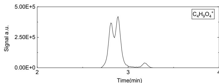
Fig. 7. Formation of KHP during DEE oxidation in a JSR. The chromatogram was recorded at m/z 121.0492 ( C_4H_9O_4^+ ) using APCI positive mode. The separation of isomers was obtained with HPLC Ascentis Silica column.
