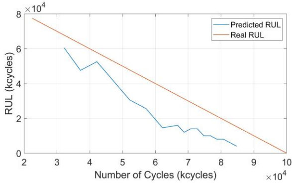
Fig.12: : Predict RUL change when applied on aging tests done under the test condition \Delta T = 90^\circ C and t_{on} = 3sec
