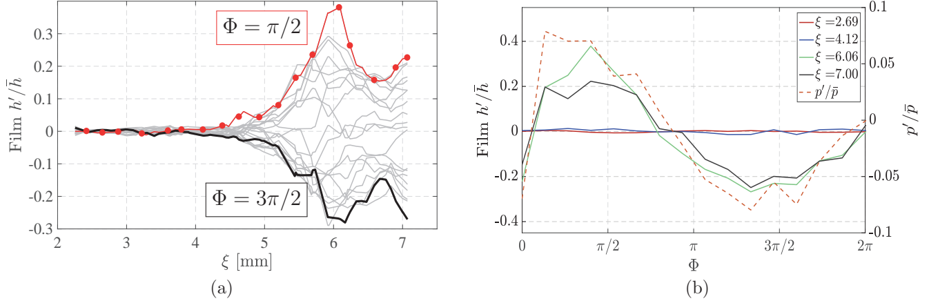
Figure 22: (a) Non-dimensional film height fluctuation, h'/\bar{h} , along the film local coordinate \xi during the period of oscillation. (b) Non-dimensional film height fluctuation, h'/\bar{h} , measured at different locations along the film, plot in phase with the mode pressure signal p'/\bar{p} properly rescaled.
