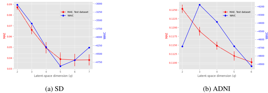
Fig. 3: WAIC score and MAE for (a) the SD dataset and (b) the ADNI dataset. In both figures, the left y-axis scaling describes the MAE while the right y-axis scaling corresponds to the WAIC score.
