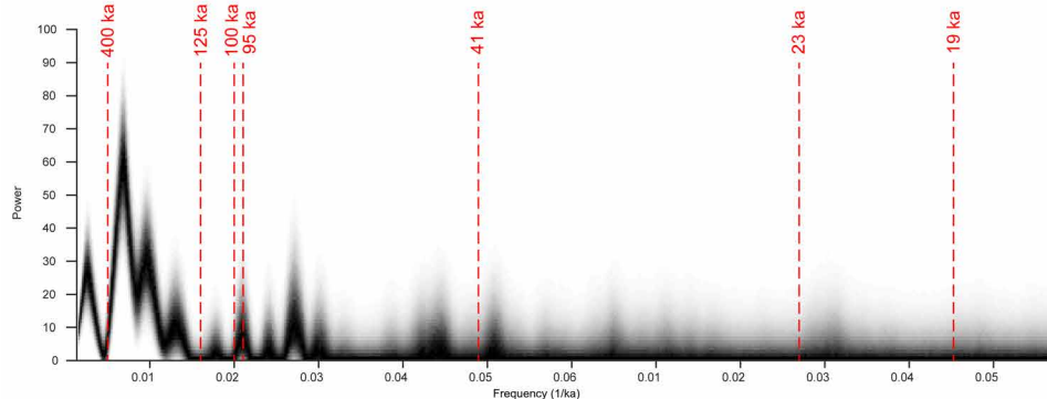
Fig. 4. Time-series (power spectrum) analyses on ODP-OLO12-1A environmental indicator (proxy) records. Lomb-Scargle spectra for (A) the diatom CA1 axis, an indicator for lake depth, (B) the XRF Si/K ratio, an indicator of paleohydrology, and (C) the phytolith D/P index, an indicator of paleovegetation and tree cover. Orbital periods (400, 100, 41, and 23 to 19 ka) are shown with red dashed lines. Spectral analysis was used to explore orbital variability within the various time series, taking into account the uncertainty of the age model (see Materials and Methods). Darker colors represent spectral powers of the data that are more consistent across the full age model. Orbital variability is present but subdued in these records: The percentage of total variance occurring at orbital periods is only 11% in the diatom CA1 record (8% eccentricity, 2% obliquity, and 1% precessional periods), 17% in the XRF Si/K time series (8% eccentricity, 7% obliquity, and 1% precessional periods), and 16% in the phytolith D/P tree cover record (9% eccentricity, 3% obliquity, and 4% precessional periods). Records are shown in comparison with orbital cycles in fig. S4.
