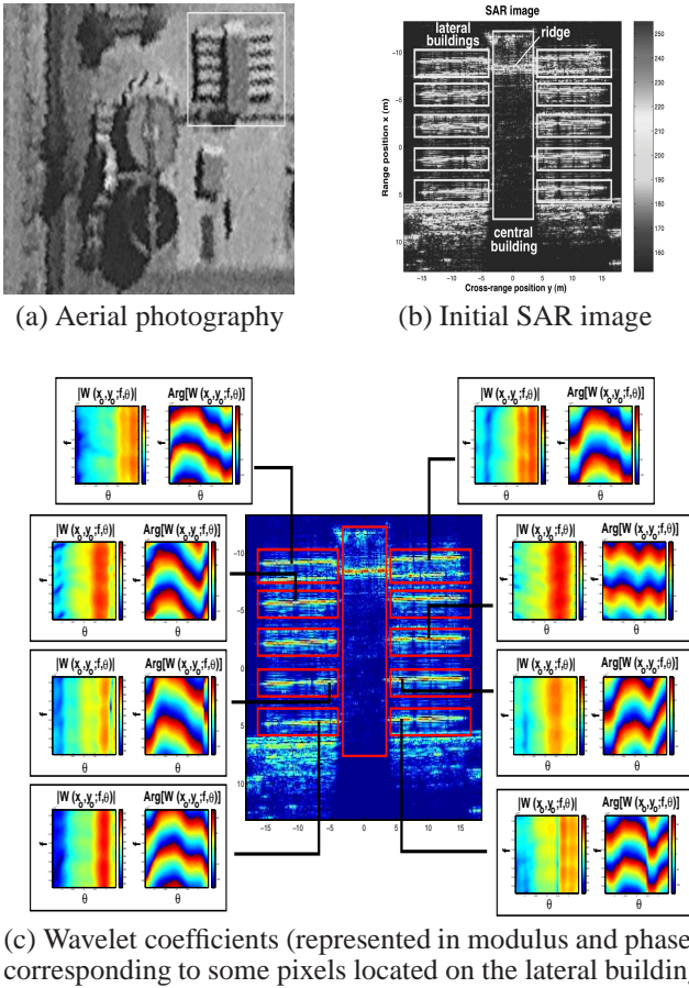
Figure 2: We reveal that the wavelet coefficients corresponding to the analysed pixels present some similarities (especially in phase).
