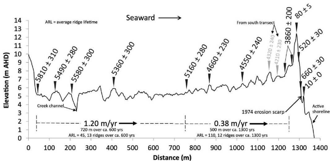
Figure 21. Shore-normal topographic profile across the centre of the Pedro Beach barrier, southeastern Australia, showing OSL ages in relation to beach ridges (lighter shaded ages are from another transect). Progradation virtually ceased nearly 3.9K years ago, to be replaced by important vertical dune ridge accretion. Adapted from Oliver et al. (2019), with permission from John Wiley and Sons.
