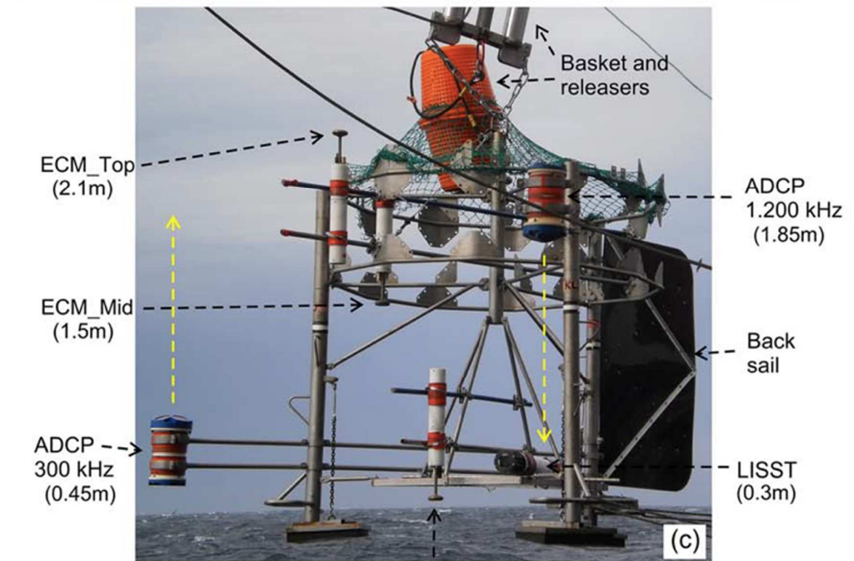
Figure 3. Photograph of a seabed lander and its instrumentation. Distance of each instrument from the bottom of the lander is also indicated. From Zhang et al. (2015), with permission from John Wiley and Sons.
