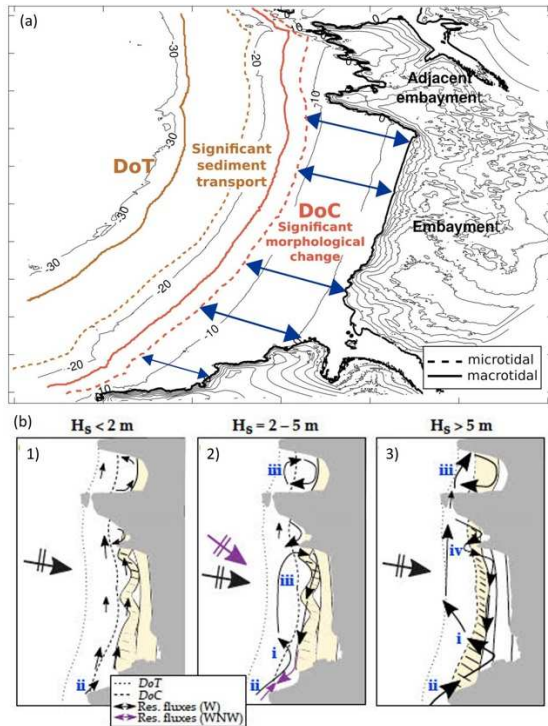
Figure 9. Plan-view showing the DoC, the DoT, and zone of significant morphological change on a 15-km stretch of the embayed high-energy macrotidal coast of north Cornwall, SW England (a); conceptual diagram showing the variability of major alongshore sediment flux pathways (b) under conditions of: 1) low waves, 2) moderate-high waves and, 3) higher than average waves. Arrows (size increases with increasing magnitude) indicate predicted residual fluxes based on Delft 3D model output. Accretion due to cross-shore fluxes is shown in beige. Dotted and dashed lines show, respectively, idealized limits of the active shoreface Depth of Transport (DoT) and Depth of Closure (DoC). (a) adapted from Valiente et al. (2019), and (b) adapted from Valiente et al. (2020), with permission from Elsevier.
