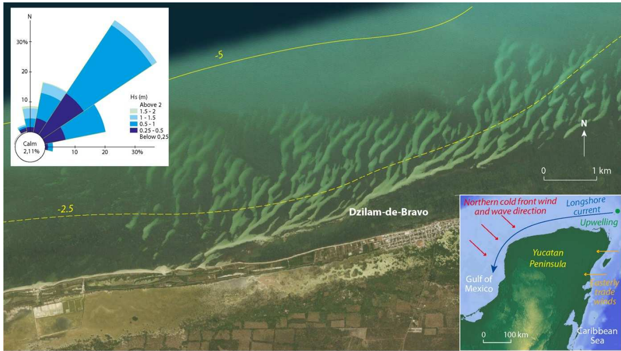
Figure 17. Google Earth image of the north coast of the Yucatan Peninsula, Mexico, showing the welding, on the US and beach, of bedforms (2-3 m high?) of carbonate sediment derived from a LS carbonate factory. Top left inset (from Appendini et al., 2012) shows wave heights measured at Dzilam-de-Bravo using an acoustic Doppler current profiler, while bottom right inset (from Lowery and Rankey, 2017) shows wind-generated hydrodynamic forcing circulation that includes significant upwelling caused by easterly winds. LS bedform mobility and onshore welding are probably driven mainly by high waves generated by cold northerly fronts. These welded forms feed the wave-driven US longshore transport system that contributes to the construction of the numerous beach ridges and spits characterizing the northern Yucatan coast.
