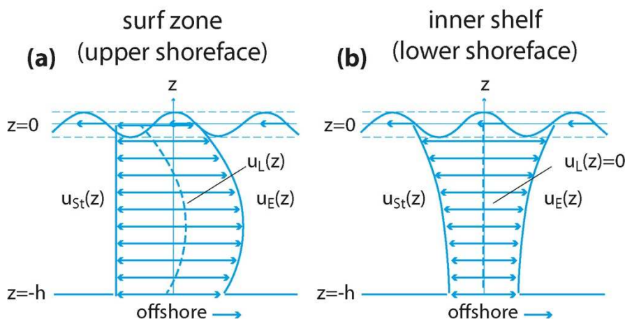
Figure 6. Two-dimensional ( x, z ) wave-driven circulation typically observed (a) inside the surf zone (US) where the onshore Lagrangian Stokes drift u_{St}(z) is uniform in depth and the offshore wave-driven Eulerian undertow u_E(z) is parabolic, resulting in a vertical imbalance in the net mean flow, u_L(z) \neq 0 (dashed line); (b) over the inner shelf (LS), where the onshore Lagrangian Stokes drift u_{St}(z) and the offshore wave-driven Eulerian undertow u_E(z) cancel,
