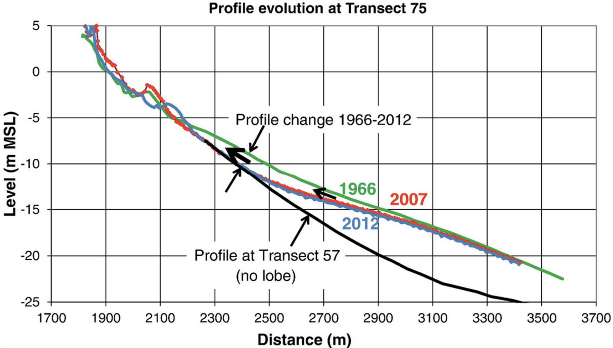
Figure 19. Progressive reworking over 46 years (1966-2012) of the abandoned delta lobe of the Nerang River, Gold Coast, Australia, on the LS, marked by onshore sand supply that significantly supplemented the longshore transport system. From Patterson and Nielsen (2016), with permission from Elsevier.
