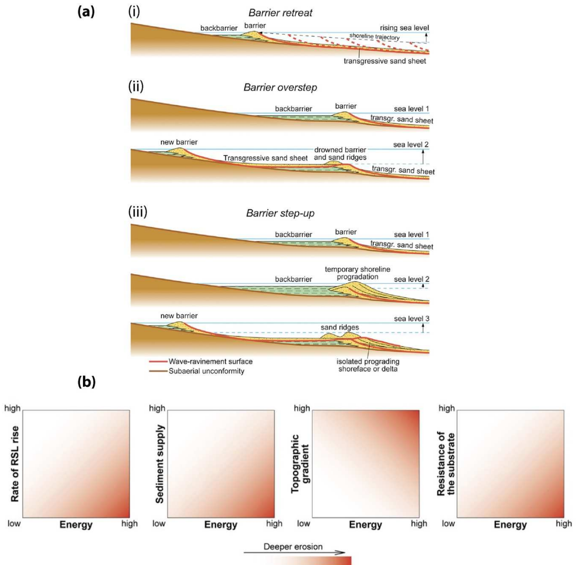
Figure 11. (a) Transgressive barrier retreat models involving a continuous landward retreat of the US resulting in the deposition of a transgressive sand sheet over the LS with its profile maintained (a1); it is worth noting that in some areas, this this sand sheet is actually a residue/lag formed by removal of certain transportable fractions; 'barrier overstep' transgressive model, where a barrier that initially retreats or grows vertically fails to keep pace with rising relative sea level and/ or does not receive enough sediment supply, resulting in barrier overstepping and a new barrier forming landward (a2); barrier mode
