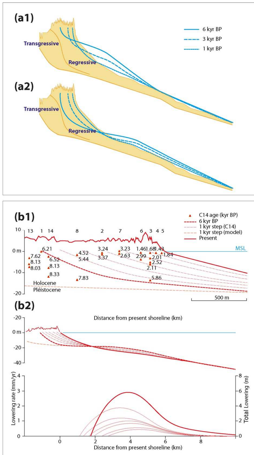
Figure 2. (a) Conceptual models proposed by Roy and Thom (1981) to explain long-term barrier progradation (regressive barriers) in response to lowering of the shoreface following the mid-Holocene sea-level stillstand: (a1) the 'sediment bulge' hypothesis, in which a barrier is supplied with sand from a convex sand body situated on the upper to middle shoreface; (a2) the 'uniform shelf lowering' hypothesis, in which sand is supplied to the barrier by near-uniform planing of the inner-shelf surface; (b) simulated strandplain growth at Tuncurry tuned to the radiocarbon chronology for stable sea-level simulations through time: (b1) 1-kyr time step shoreface surfaces interpreted from C14 chronology; (b2) simulated underlying shoreface sand supply driven by disequilibrium morphology (81%) with
