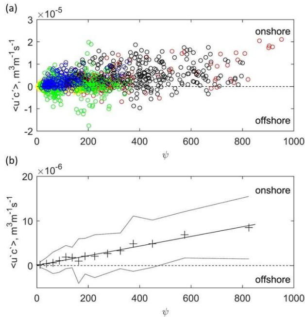
Figure 7. Wave-driven (oscillatory) transport ( u'c' ) as a function of the mobility number, \psi . Panel (a) shows measured transport rates on the LS at Vejers Beach, Denmark (red symbols), Fanoe Beach, Denmark (black symbols), Pearl Beach, NSW, Australia (green symbols), Staengehus Beach, Denmark (blue symbols) and Skallingen, Denmark (yellow symbols). Panel (b) shows the average transport rates within separate \psi -bins. The best-fit relationship (solid line) has an R^2 = 0.968 and a root-mean-square error of 1.651 \cdot 10^{-6} . The dotted lines indicate \pm 1 standard deviation about the means. From Aagaard (2014), with permission from John Wiley and Sons.
