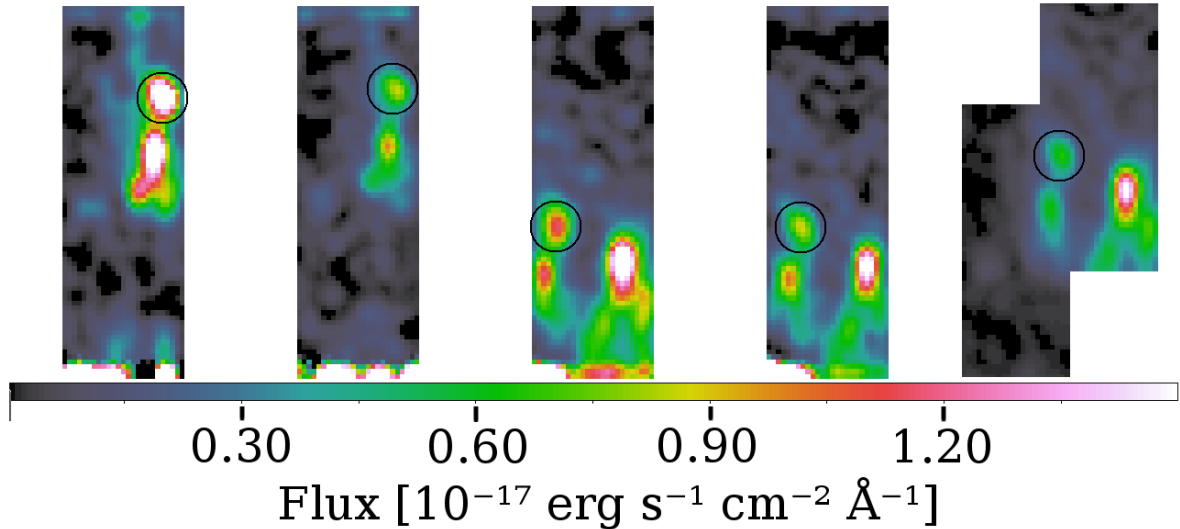
Fig. 2. Colour-scale images in the four left panels show the plane with H\alpha emission in the four single data cubes of the southern pointing of ESO111-G014. The black circles indicate the feature that was used to align the four data cubes. Right panel : plane with H\alpha emission in the final, stacked data cube.
