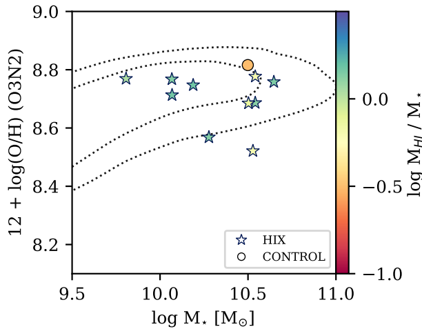
Fig. 5. Mass–metallicity relation for the H I X galaxies: we show the gas-phase metallicity (determined with the O3N2 parameter following Pettini & Pagel 2004) as a function of stellar mass. The contours enclose 64 and 90% of SDSS galaxies. The circle indicates the CONTROL galaxy IC 4857 and H I X galaxies are marked with stars. All symbols are also colour-coded by the H I mass fraction.
