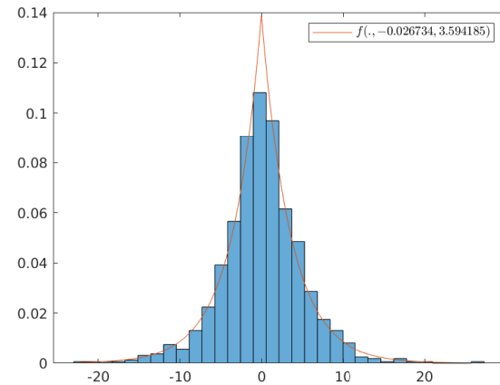
(b) Normalized histogram and Laplacian fitting.
