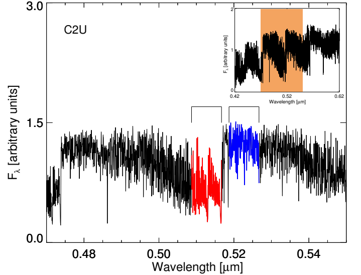
Fig. 13. The C 2 Swan system (top panel) and a zoom into the C 2 line around 0.5165 \mu\text{m} . The red line indicates the region used to calculate the C 2 U_band bandpass, while the blue line corresponds to the C 2 U_cont bandpass measuring the continuum. This star is HE 1428-1950.
