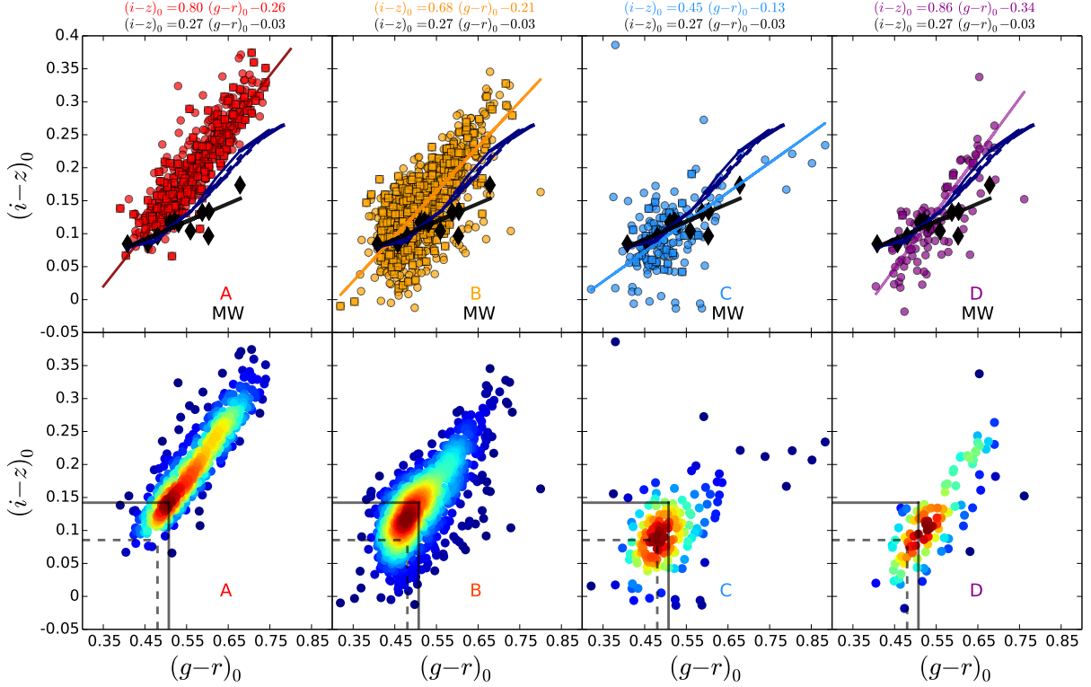
FIG. 2.— (g-r)_0 versus (i-z)_0 color-color diagram for different GC samples. ( Top panels ): Comparison of various NGVS GC sub-samples (from left to right: A , B , C , D ), with MW GCs (black diamonds). Circles and squares mark GCs without and with radial velocity information. Linear ML-fits to the NGVS-GC sub-samples and MW GCs are given in the top of each panel. In addition, we show SSP predictions taken from the Bruzual & Charlot (2003) model for metallicities 0.0002 < Z < 0.03 and ages 6 < t < 13 Gyr. All colors are de-reddened with extinction values taken from Schlegel et al. (1998). ( Bottom panels ): Corresponding density plots for the NGVS GC sub-samples highlighting the colors of the highest-density peaks and their shift from the A GCs toward the C sample, illustrated by solid and dashed lines, respectively.
