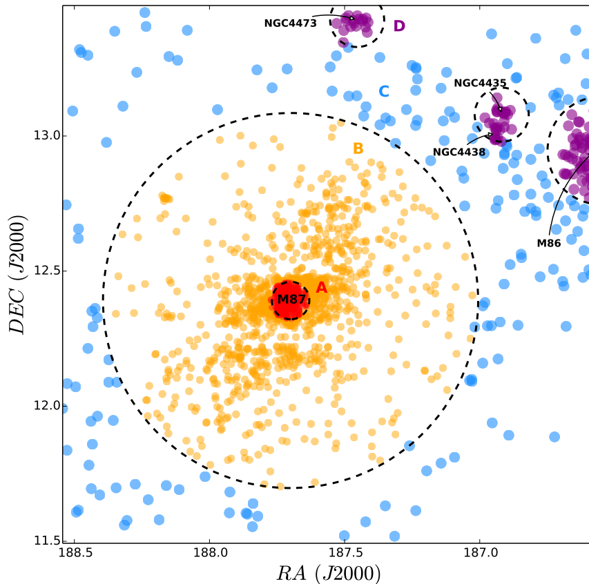
FIG. 1.— Spatial distribution of the NGVS GC sub-samples. The red GCs are located within a projected radius of 20 kpc from the M87 center. The orange points show GCs between 20 \leq r < 200 kpc. The blue GCs are defined by r > 200 kpc and being not associated with the M86, NGC 4435, NGC 4438 and NGC 4473. GCs associated with the latter galaxies are indicated by magenta points.
