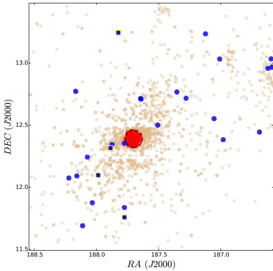
FIG. 4.— Spatial distribution of the GC sub-samples defined in Fig 3.
