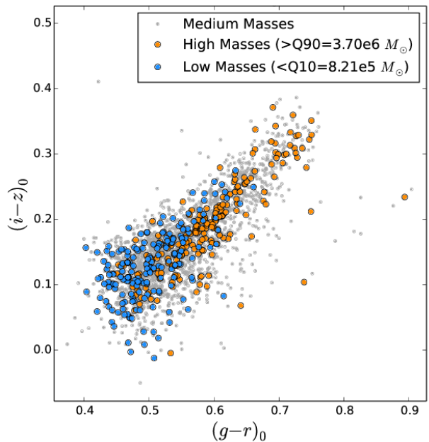
FIG. 5.— (g-r)_0 versus (i-z)_0 color-color diagram for three GC samples selected by their masses which provides evidence that mass is not the driving factor in the difference between Virgo GCs in subset E or elsewhere.
