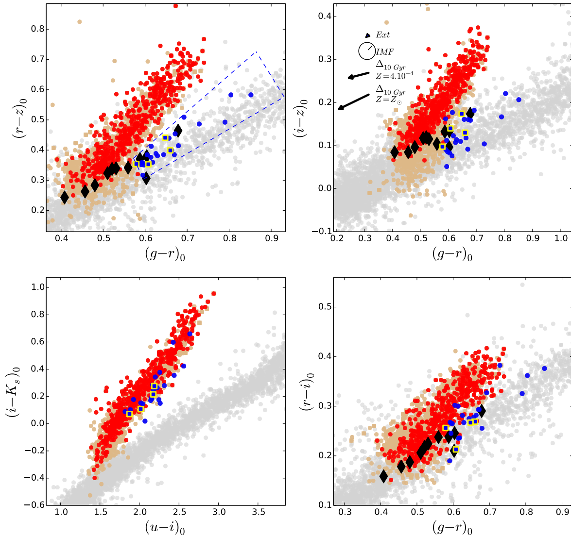
FIG. 3.— Color-color diagrams comparing the NGVS sample (colored dots, see Figure 1 for the definition of subsets) and the MW GCs (black diamonds). GCs within 20 kpc from the M87 center are highlighted in red and GCs from subset E in blue, four of which are radial-velocity confirmed and marked with yellow contours. The NGVS foreground stars are shown in grey. Circles and squares mark GCs without and with radial velocity information consistent with Virgo cluster membership, respectively. In the top right panel, vectors illustrate the shifts induced by several systematic changes.
