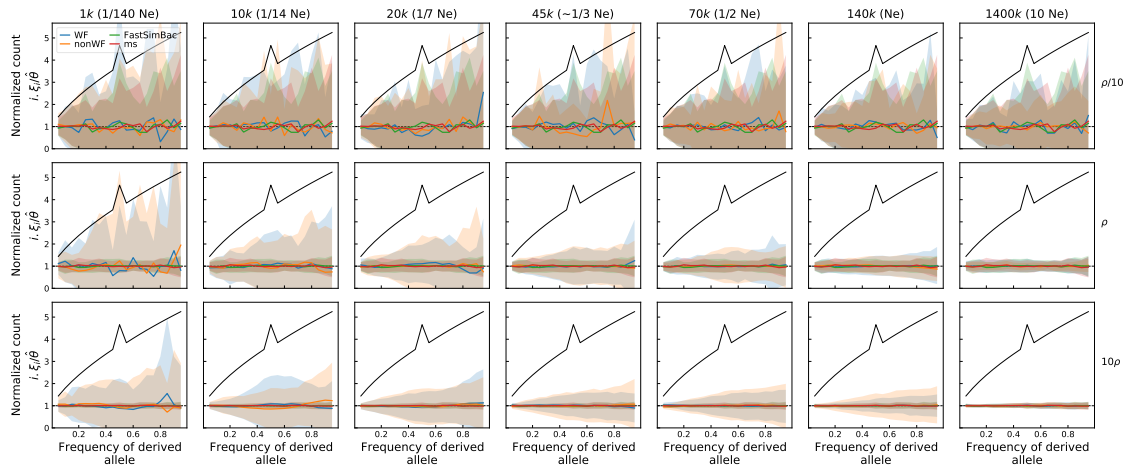
Figure S5: The normalized Site Frequency Spectrum (SFS) for different numbers of forward-simulated generations and recombination rates. The number of generations are indicated on the top of each column (e.g. 1k is 1,000 generations, and corresponds in unit of N_e to 1/140-th of N_e ). The shaded areas represent standard deviation. The black lines represent the expected standard deviation for the Wright-Fisher model without recombination. N_e=140\,000 , \lambda = 12200\text{bp} and \text{RF}=25 .
