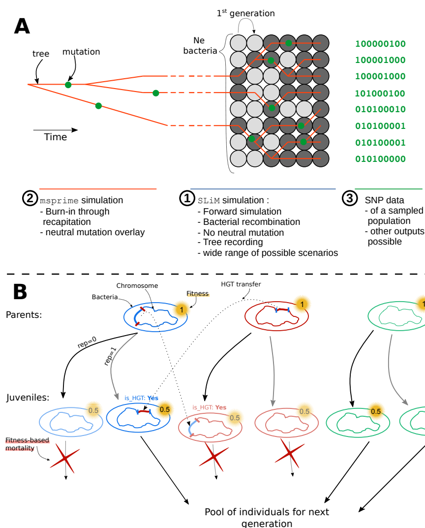
Figure S1 – Schema of the nonWF simulation process described in this study. This schema is a visual companion to section 2.2 Simulation protocol, and is not self sufficient. (A) Step ①: forward simulation with SLiM of a population of bacteria with N_e individuals. The population at the time of sampling (on the right-hand side) will not have coalesced, here, for example, there are still three ancestors at the first generation (darker circles) and no single most recent common ancestor. Step ②: burn-in with msprime by recapitation of the tree sequence. The recapitation coalesces remaining branches back in time, acting as a burn-in period for the forward simulation. Then we can overlay neutral mutations on the fully coalesced tree sequence. Step ③: output SNP data for further analysis. Other types of data may be output, such as a VCF file, or a .trees tree sequence file. Panel (B) provides a simplified depiction of the reproduction process. Each parent produces two juveniles, and some of them will receive gene fragments (thicker chromosomal segments) from other parents by HGT. Parents that are going to receive HGT are drawn from a binomial distribution with the HGT rate as the probability (HGT rate parameter, L. 36 in the bacterial reproduction code snippet). The first position of the recombining fragment is drawn uniformly along the chromosome, and the second position is drawn from a geometric distribution with the mean tract length parameter (tract len parameter, L. 50). The fitness is then adjusted by density-dependent selection, causing mortality (red crosses), such that on average the population size remains constant at equilibrium (see Regulating the population size's code snippet, L. 81- 92).
