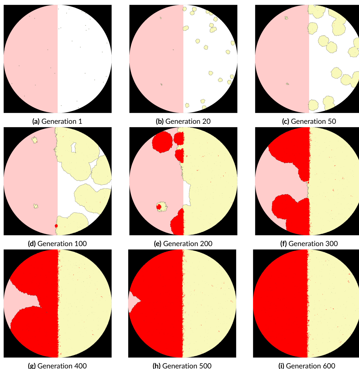
Figure 7 – Representation of the simulated Petri dish at different generations. The pink area represents the half of the dish with antibiotic, while the white half has none. At the first generation, there are 50 colonies (single bacteria) spread randomly on the plate. As the simulation goes forward, we see those colonies growing, in yellow. They grow better in the right-hand half of the plate, due to the absence of antibiotic. Bacteria colored red have acquired antibiotic resistance. We see that the resistant bacteria later grow better in the left half of the dish. Because of the fitness cost of the antibiotic-resistance mutation in the absence of antibiotic, there are only a few red bacteria in the right half at the end of simulation despite their markedly higher mean fitness over the environment as a whole, showing the importance of spatiality for the outcome of the model. The code used to generate this simulation can be found at https://github.com/jeanrjc/BacterialSimulations .
