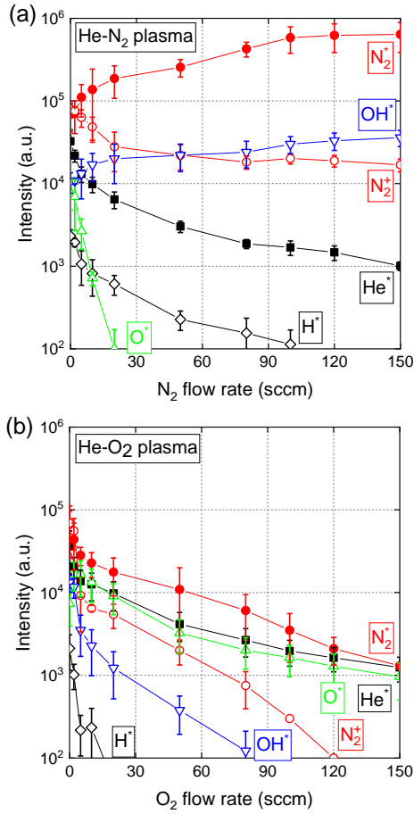
Figure 5. Optical emission of plasma radiative species as a function of (a) N 2 flow rate or (b) O 2 flow rate. In all cases, the reactive gas (N 2 or O 2 ) is mixed with 2 slm of helium; all measurements are achieved in SP-DBD configuration.
