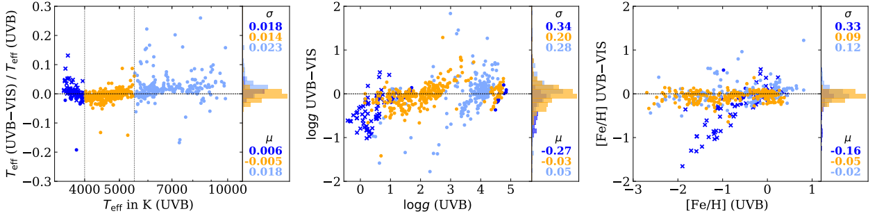
Fig. 6. Difference between the parameters determined from the UVB and VIS spectra for stars with 3500 \text{ K} < T_{\text{eff}} (\text{UVB}) < 10000 \text{ K} . The colour-coding is the same as in Fig. 5, and for the coolest stars ( < 4000 \text{ K} ) the giants are shown with crosses. In the \log g panel, two outliers (hot stars) are not shown. The dispersion \sigma and mean offset \mu for the three temperature ranges are indicated.
