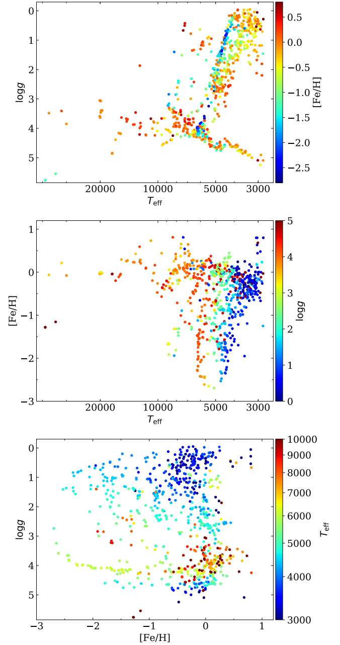
Fig. 7. Final parameters in this paper for XSL. Top panel: Hertzsprung-Russell diagram for XSL, colour-coded by [Fe/H]. Middle: distribution in the T_{\text{eff}} - [\text{Fe}/\text{H}] plane, colour-coded by \log g . Bottom: distribution in the [Fe/H] – \log g plane, colour-coded by \log T_{\text{eff}} . One star with a \log g error larger than 2.0 is not shown (carbon star [ABC89] Cir 18).
