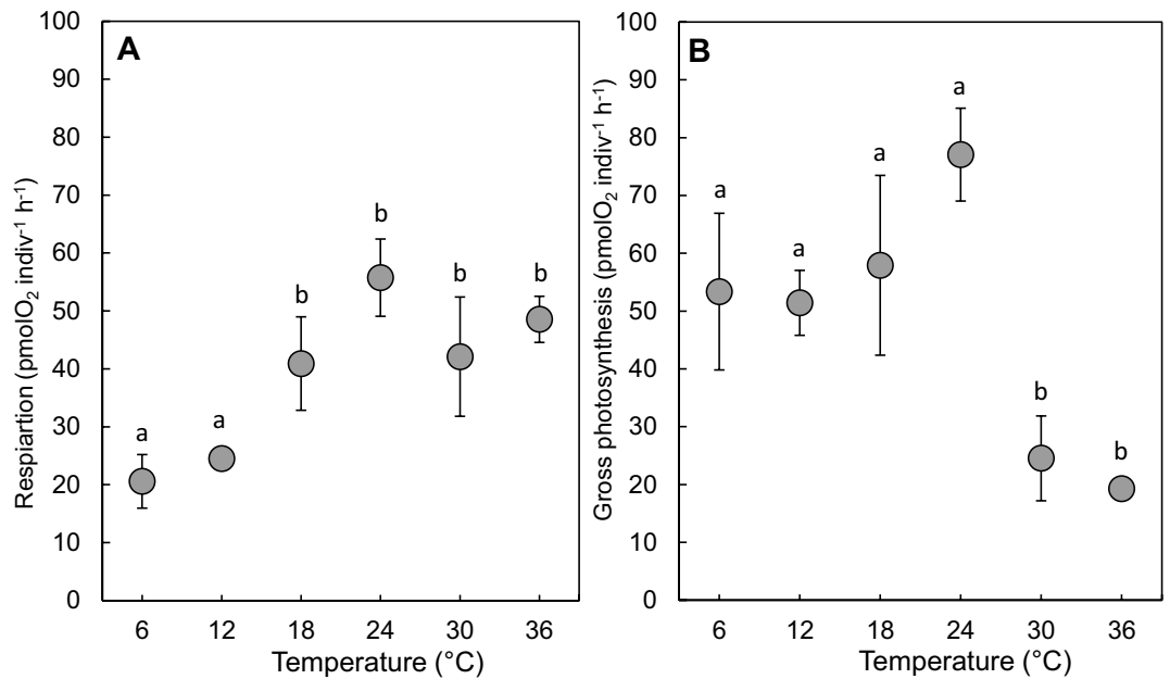
Figure 5. Mean values of (A) respiration and (B) gross photosynthesis (pmolO 2 indiv -1 h -1 ) of H. germanica under different thermal regime in 3 replicate measurements. The error bars are the standard errors of the mean. Letters ‘a’ and ‘b’ identify significant different groups (Tukey test, p < 0.05 ).
