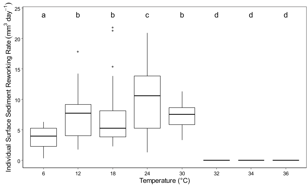
Figure 6. Individual surface sediment reworking (mm³ indiv⁻¹ day⁻¹) of H. germanica under different thermal regime. Letters above plots ('a', 'b', 'c') indicate significant differences among measurements (Dunn test, p < 0.05 ). The box represents the first, second and third quartiles and the whiskers extend to 1.5 times the interquartile range; values outside this range are represented by open circles.
