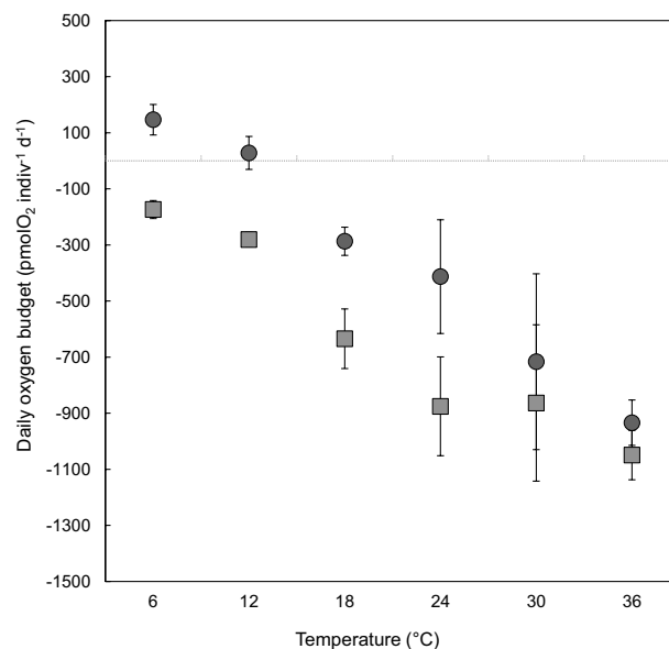
Figure 7. Daily oxygen budget of H. germanica (pmolO₂ indiv⁻¹ day⁻¹) under 12 h (black dots) and 6 h (grey squares) light exposure and thermal regimes. The error bars are the standard errors calculated on the 3 replicates at each temperature.
