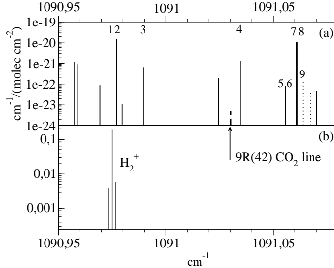
FIG. 1: (a) Full lines : HCOOH lines of intensity larger than 10^{-23} \text{ cm}^{-1}/(\text{molec cm}^{-2}) from HITRAN 2004 database [8]. Dotted lines : additional lines predicted by A. Perrin [17]. The numbering of the HCOOH lines corresponds to that given in the last column of Table I. When operated on the 9R(42) \text{CO}_2 line, the \text{CO}_2/\text{HCOOH} reference laser is stabilized on line n°4. (b) (v=0, L=2) \rightarrow (v=1, L=2) \text{H}_2^+ two-photon transition spectrum in atomic units, see ref. [4]. The central peak is a 6.5 MHz wide doublet.
