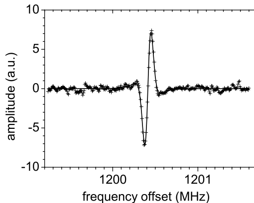
FIG. 4: Third harmonic phase sensitive saturated absorption signal of HCOOH at 32 707 063 566.1 kHz, labelled 3 in the last column of Table I versus the frequency offset 8\delta between the reference laser and the phase locked QCL (see Fig. 3). The integration time is 1 s per point. Full line: adjustment by a third Lorentzian derivative. The full width at half maximum is 220 kHz.
