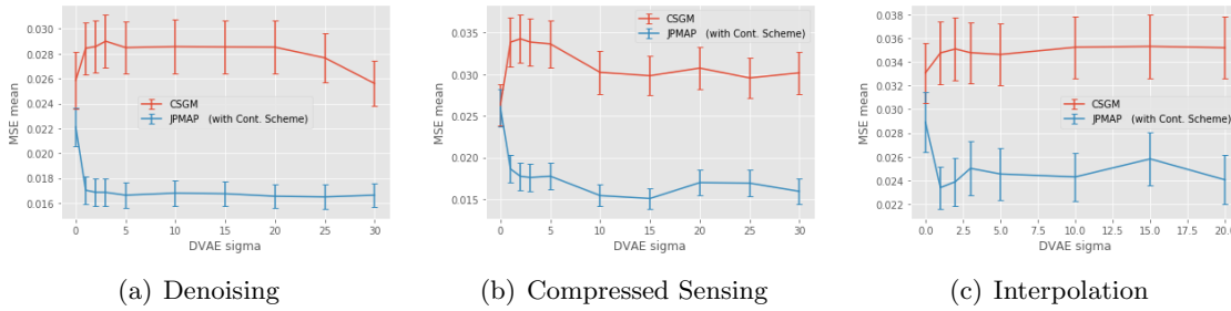
Figure 2. Evaluating the effectiveness of JPMAP vs CSGM as a function of \sigma_{\text{DVAE}} (same setup of Figure 1). Without a denoising criterion \sigma_{\text{DVAE}} = 0 the JPMAP algorithm may provide wrong guesses \mathbf{z}^1 when applying the encoder in step 2 of Algorithm 2.2. For \sigma_{\text{DVAE}} > 0 however, the alternating minimization algorithm can benefit from the robust initialization heuristics provided by the encoder, and it consistently converges to a better local optimum than the simple gradient descent in CSGM.
