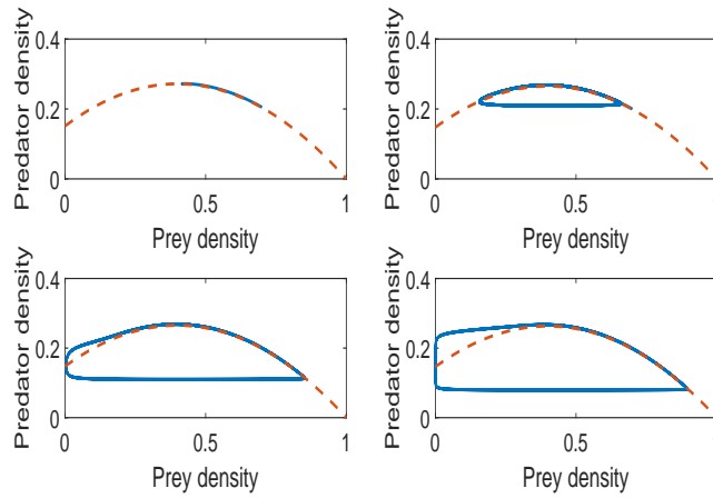
Fig. 6 Several phase portraits showing the birth of the limit cycle in the Hopf bifurcation with a canard phenomenon. On the top left panel, an equilibrium point close to the top of the parabola is globally asymptotically stable. On the top right panel, just after the Hopf bifurcation, a small limit cycle is present. On the bottom left panel, the limit cycle amplitude is drastically enlarged (canard explosion) while the bifurcation parameter is still very close to the value used on the top right panel. Note that the trajectory remains along the unstable branch of the parabola during a finite time. On the bottom right panel, the limit cycle is the largest one. The parameter values used for these simulations are b = 0.2 , m = 0.9 and \lambda = -0.05 in top-left, \lambda = 0.0112 in top-right, \lambda = 0.01123 in bottom-left and \lambda_1 = 0.03 in bottom-right. For each panel, \varepsilon = 0.02 .
