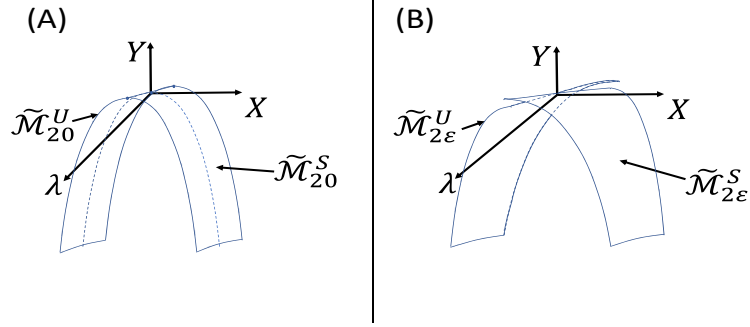
Fig. 1 Scheme of the invariant manifolds \mathcal{M}_{2\varepsilon} for \varepsilon = 0 (A) and for \varepsilon > 0 and small (B).
