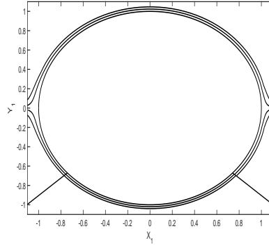
Fig. 4 Simulation of the vector field on the blown-up object in the phase plane \varepsilon = 0 and \lambda_1 = 0 . Simulations have been made in each chart and then the trajectories have been mapped onto the blown up object. The full circle is the equator of the hemisphere
