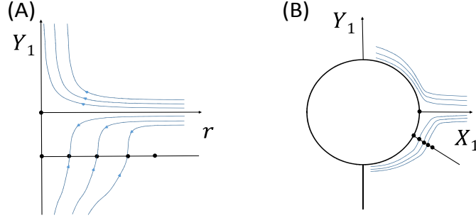
Fig. 3 Scheme of the dynamics in a chart \{X_1 = 1\} for \varepsilon_1 = 0 and \lambda_1 = 0 , given by system (7) (panel (A)). Panel (B) illustrates the transformation of the dynamics around the hemisphere in the plane \varepsilon_1 = 0 and \lambda_1 = 0 , provided by the study in the previous chart \{X_1 = 1\} . Black points correspond to equilibria.
