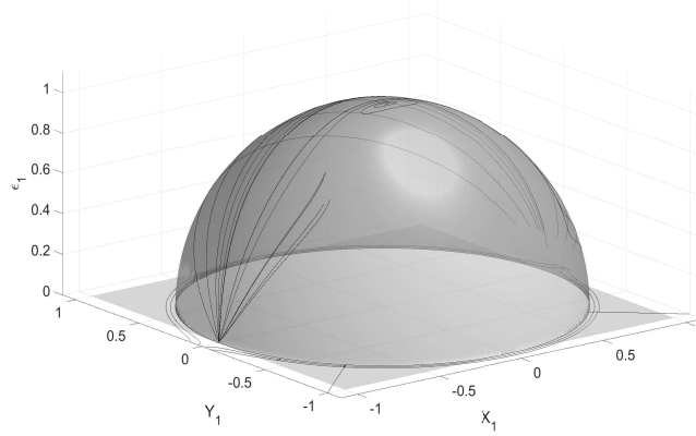
Fig. 2 Scheme of blow-up around the singularity (0,0,0,0) for a fixed positive \lambda .
