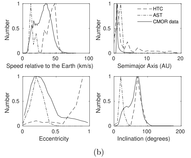
Fig. 9. Modelled impact speed and orbital elements at Earth for the apex (a) and toroidal (b) categories, compared to CMOR data, for F_{\text{coll}} = 30 and mass distribution \alpha = 5, \beta = 2 , and D_{\text{mid}} = 100 \mu\text{m} .
