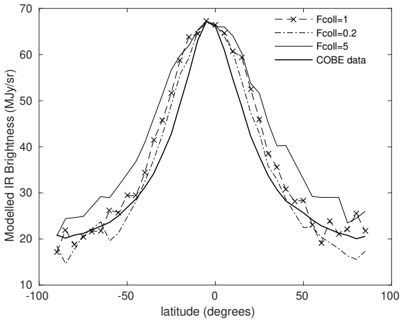
Fig. 4. Modelled infrared brightness profiles for JFCs for F_{\text{coll}} = 1, 0.2, and 5 , compared to the COBE 25 \mu\text{m} brightness profile at a solar longitude of 90^\circ . Mass distribution \alpha = 5 , \beta = 2 , D_{\text{mid}} = 200 \mu\text{m} .
