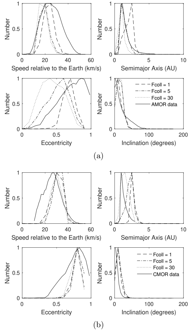
Fig. 6. Modelled impact speed and orbital elements at Earth for JFC meteoroids for the helion category, compared to AMOR (a) and CMOR (b) data, for F_{\text{coll}} = 1, 5, \text{ and } 30 , and mass distribution \alpha = 5, \beta = 2 , and D_{\text{mid}} = 200 \mu\text{m} .
