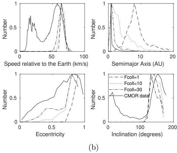
Fig. 7. Modelled impact speed and orbital elements at Earth of HTC meteoroids for the apex category, compared to AMOR (a) and CMOR (b) data, for F_{\text{coll}} = 1, 10, \text{ and } 30 , and mass distribution \alpha = 5, \beta = 2 , and D_{\text{mid}} = 200 \mu\text{m} .
